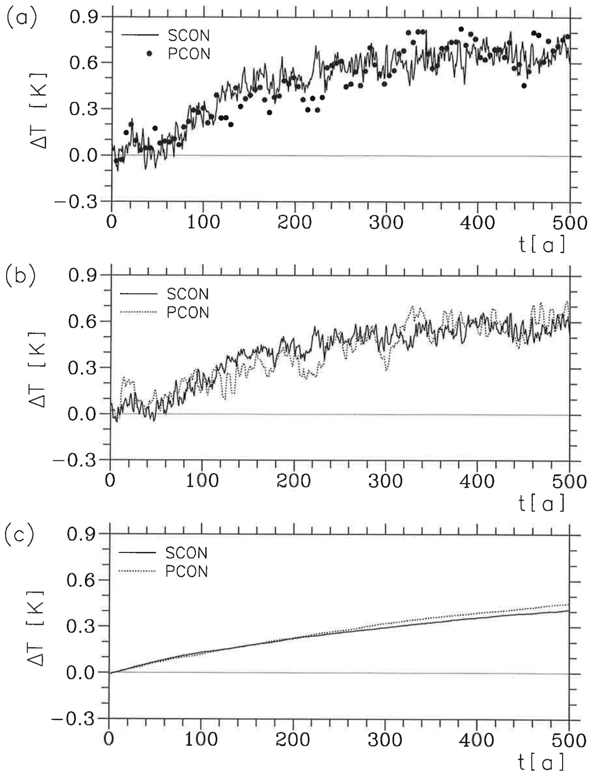
Figure 3: Time evolution of the anomalies of the global mean near surface air temperature (a), the global mean ocean temperatures for the uppermost ocean layer (25 m) (b), and for the model layer centred in 2000 m depth (c). The respective means of the first decade of the experiment SCON are subtracted. The dots in (a) indicate the means of the last 12 months of the synchronously coupled periods of the experiment PCON.
