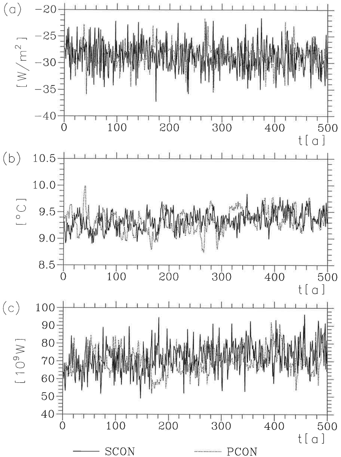
Figure 12: Time evolution of the heat flux (a), the oceanic temperature of the uppermost ocean layer (b), and the loss of potential energy by convection (c). The time series consist of annual mean averages over the North Atlantic (north of 30^{\circ}\text{N} ).
