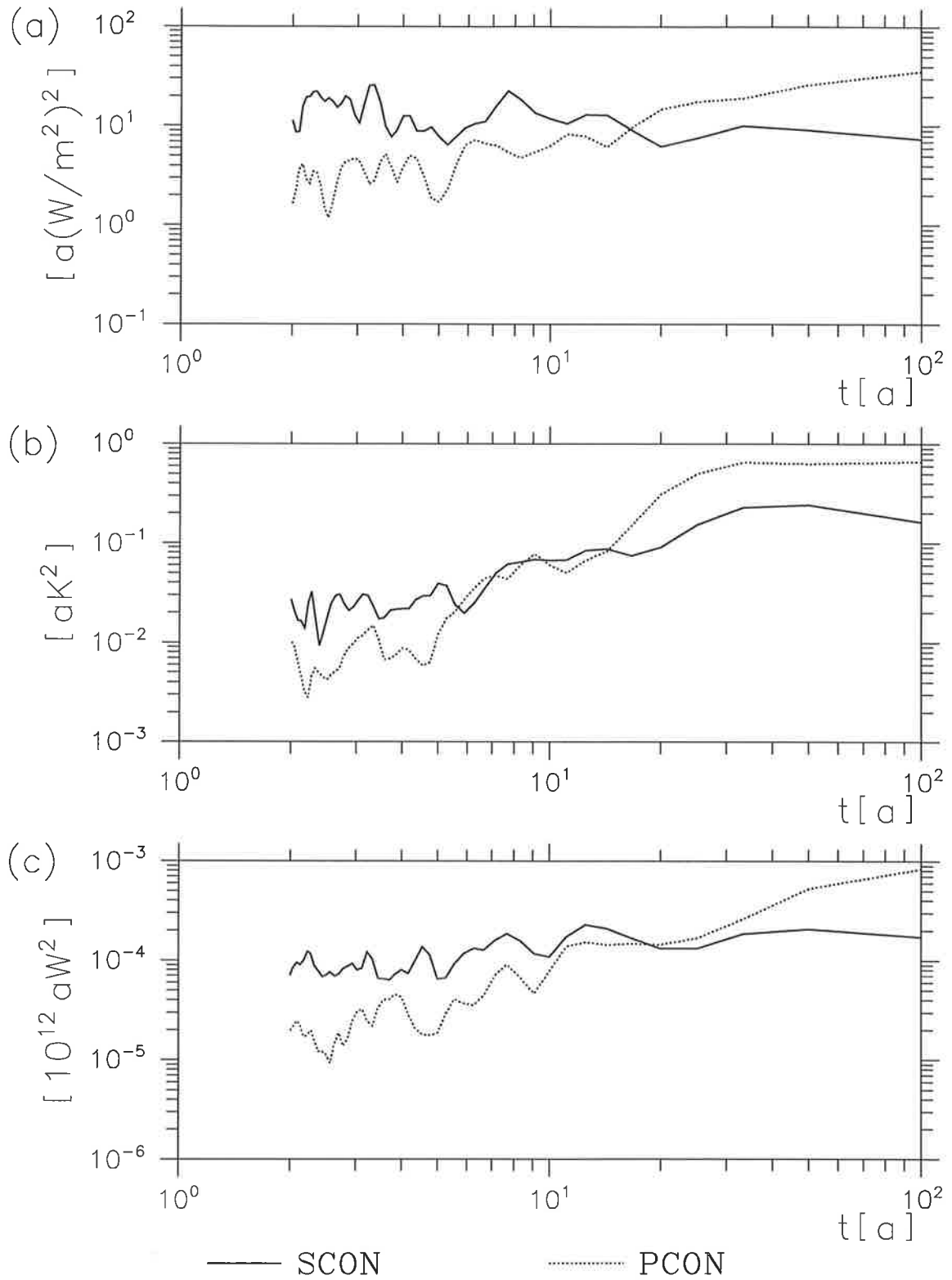
Figure 13: Spectra of the time series for the North Atlantic displayed in Figure 12. The shown variables are heat flux (a), oceanic temperature of the uppermost ocean layer (b), and loss of potential energy by convection (c). The spectra are calculated by means of the autocovariance function using a Hanning window with a maximum lag of 100 years.
