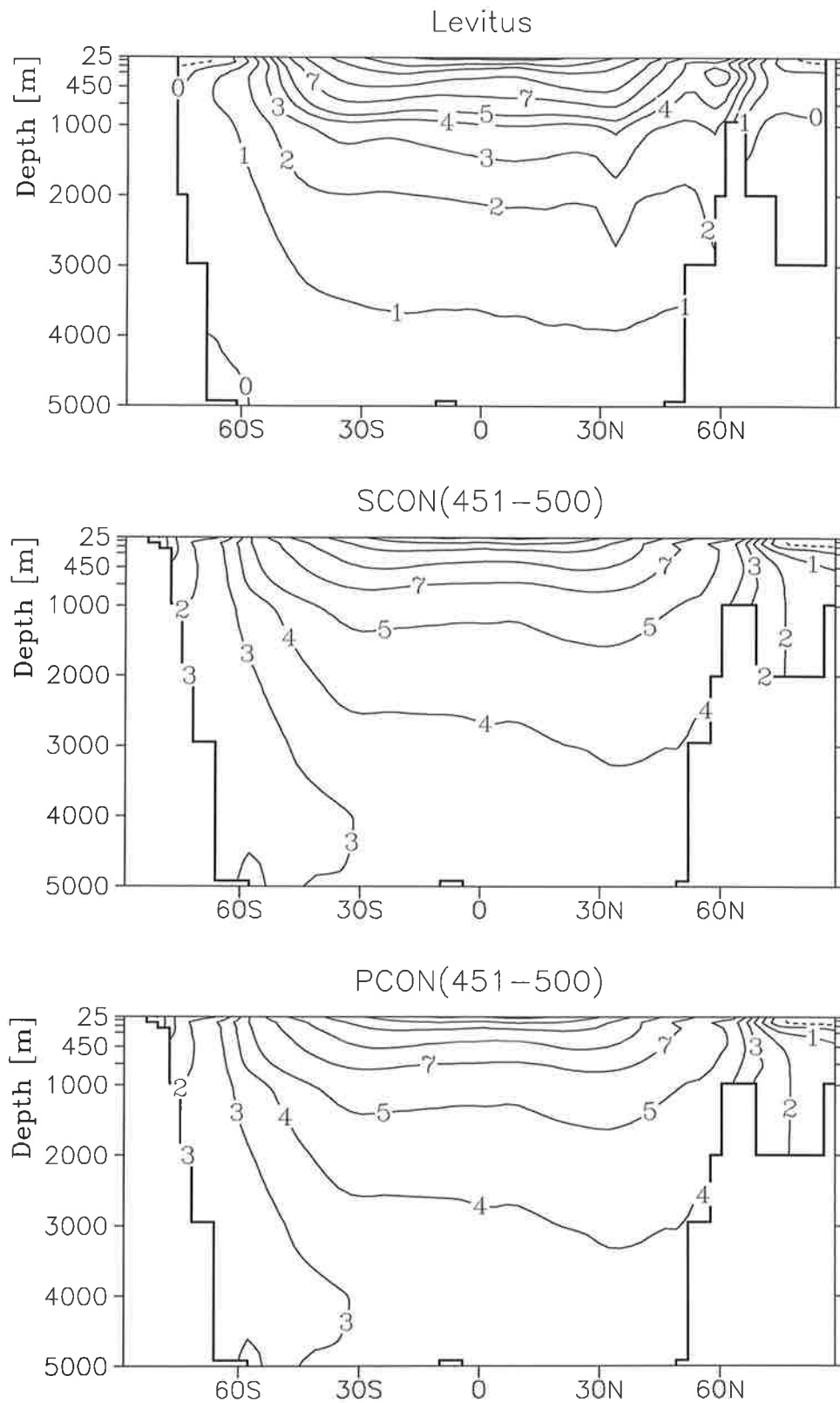
Figure 7: Zonal mean ocean temperature [°C] for observations (upper panel; Levitus, 1982) and the mean distributions of the period 451 - 500 for the experiments SCON (middle panel) and PCON (bottom panel). Contours for -1, 0, 1, 2, 3, 4, 5, 7, 10, 15, 20, 25 °C.
