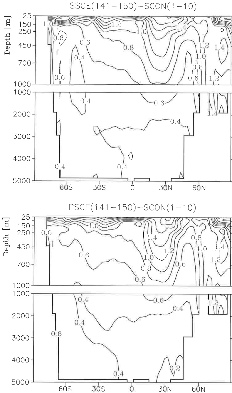
Figure 18: Anomalies of the zonal mean ocean temperatures [K] for the Atlantic. The values of the period 141 - 150 of the experiments SSCE (upper panel) and PSCE (bottom panel), respectively, are related to the means of the first decade of the experiment SCON.
