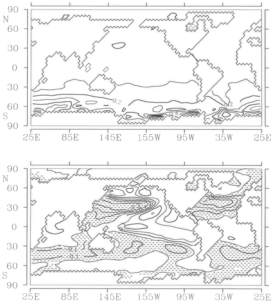
Figure 10: Pattern of the first (upper panel) and the second EOF (bottom panel) of the annual mean temperatures of the uppermost ocean layer for the experiment SCON.
