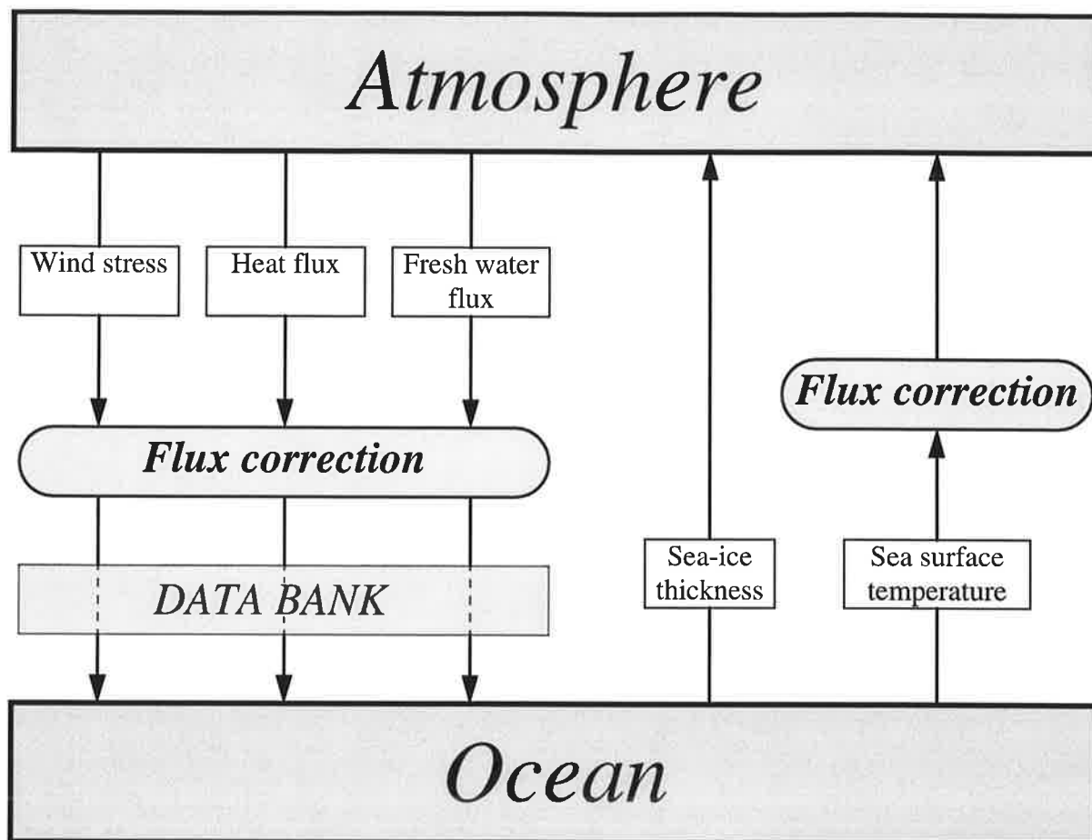
Figure 1: Coupling of the atmosphere model ECHAM3 with the ocean model LSG.
