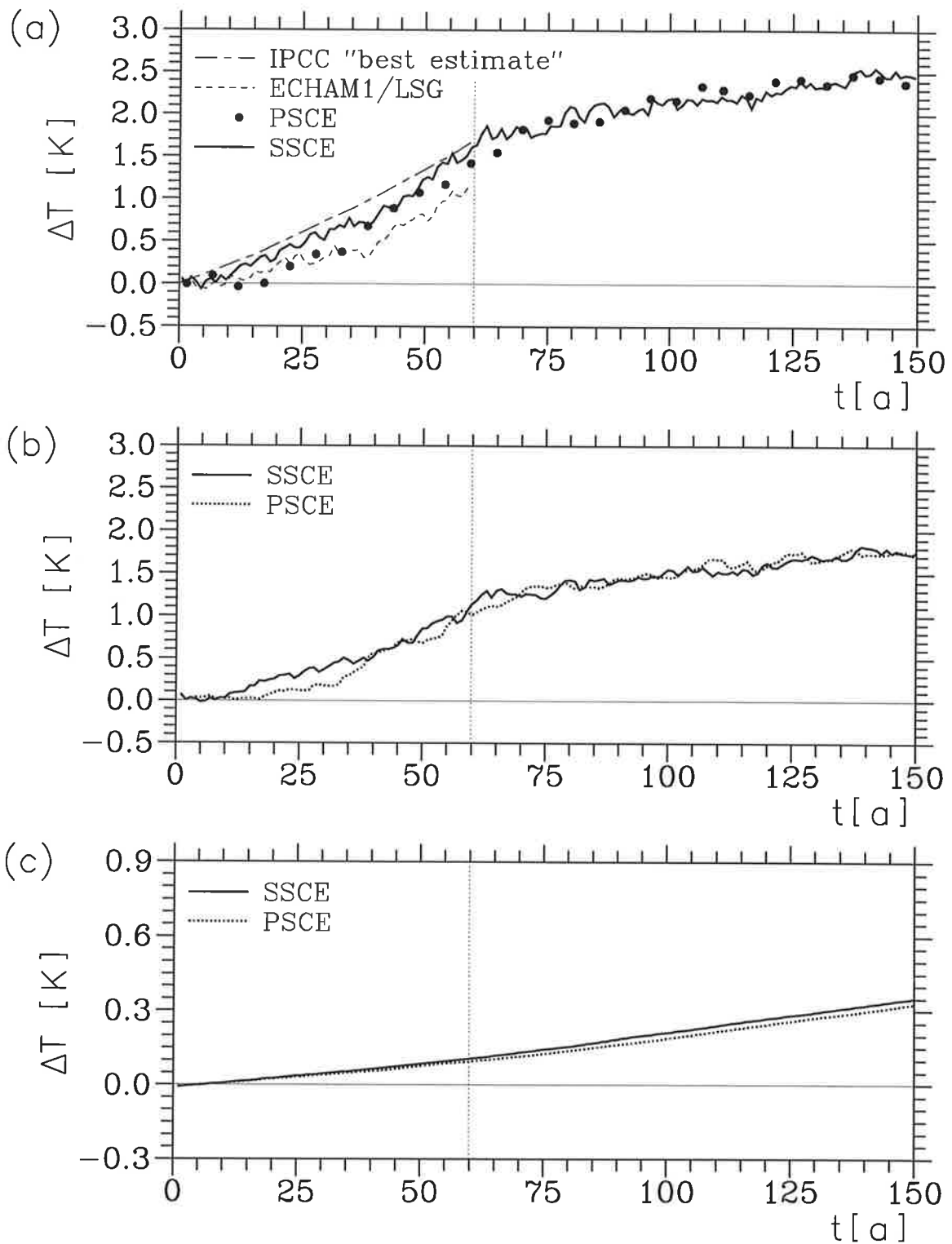
Figure 14: Response of the global mean near surface air temperature (a) and the global mean oceanic temperatures of the uppermost ocean layer (b) and the model layer centred in 2000 m depth (c). The means of the first decade of the experiment SCON are subtracted. In addition in (a) the corresponding estimate of the IPCC (Houghton et al., 1990) and the corresponding experiment of the ECHAM1/LSG AOGCM (Cubasch et al., 1992) are shown.
