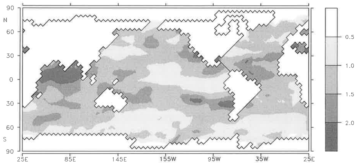
Figure 9: Ratio of the standard deviations (PCON : SCON) of the annual mean temperatures of the uppermost ocean layer for the period 451 - 500.
