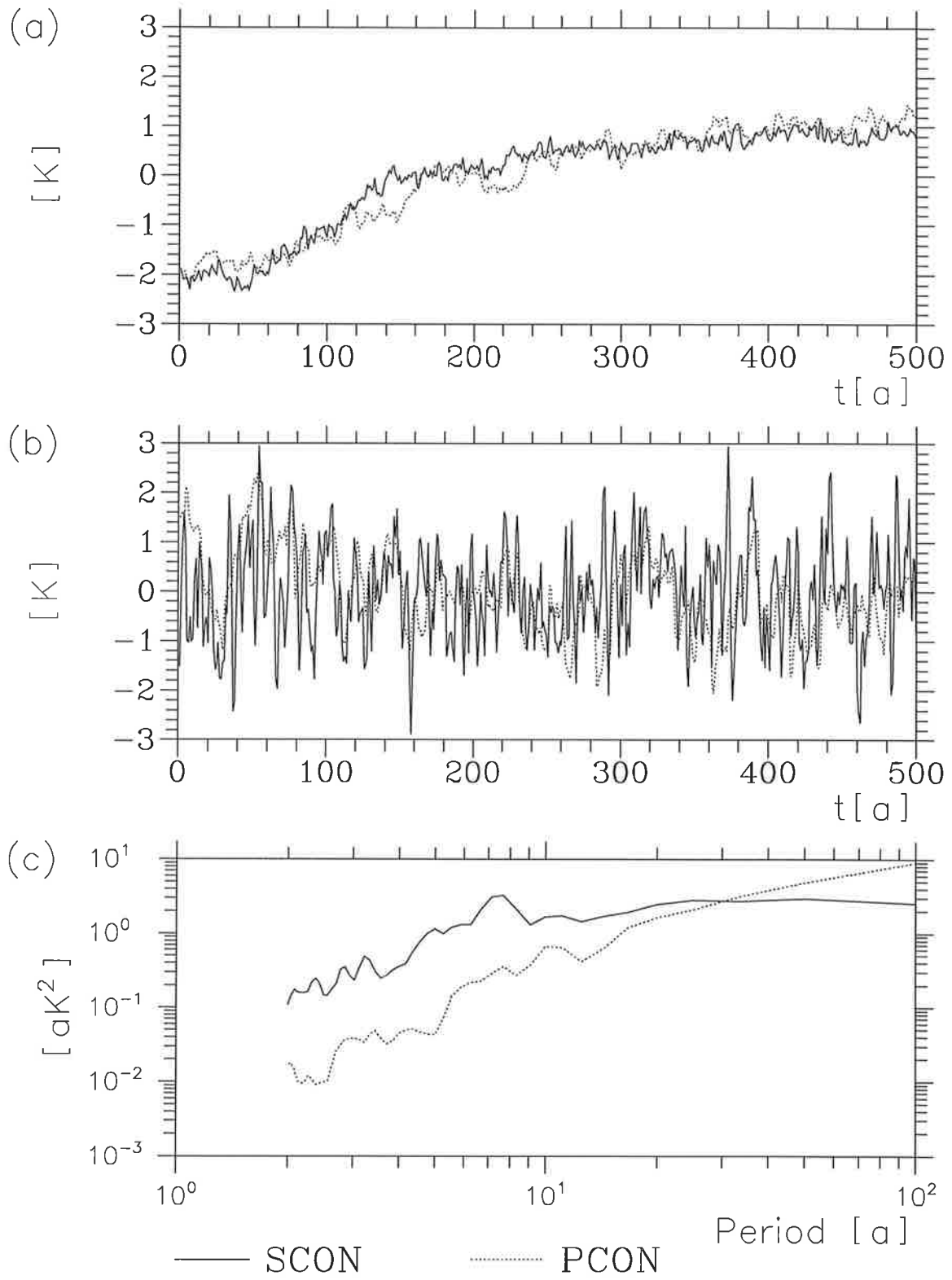
Figure 11: Time series of the principal components of the first (a) and second EOF (b) of Figure 10 and the corresponding spectra for the time series of the second EOF (c). The spectra are calculated by means of the autocovariance function using a Hanning window with a maximum lag of 100 years.
