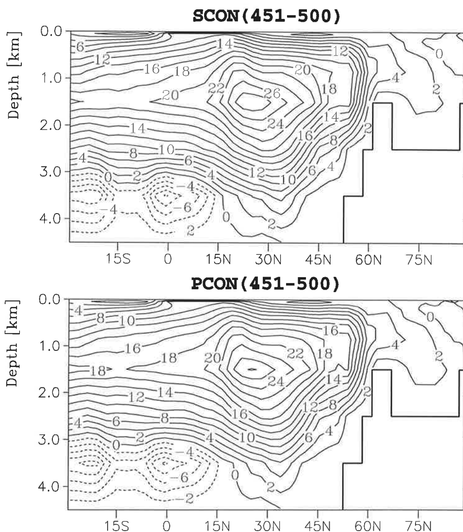
Figure 8: Meridional stream function of the Atlantic [Sv] for the experiments SCON (upper panel) and PCON (bottom panel). Displayed are the means for the period 451 - 500. Positive values indicate a clockwise rotation.
