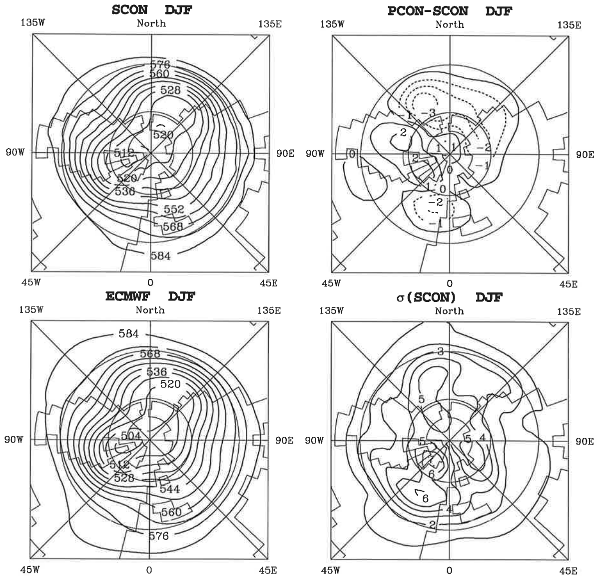
Figure 6: Distributions of the geopotential height field in 500 hPa [gpdam] of DJF for the period 451 - 500 of the experiment SCON (left upper panel), the analysis of the ECMWF (left bottom panel), the differences between the period 451 - 500 of the experiments PCON and SCON (right upper panel), and the standard deviations of the seasonal mean values of the experiment SCON (right bottom panel).
