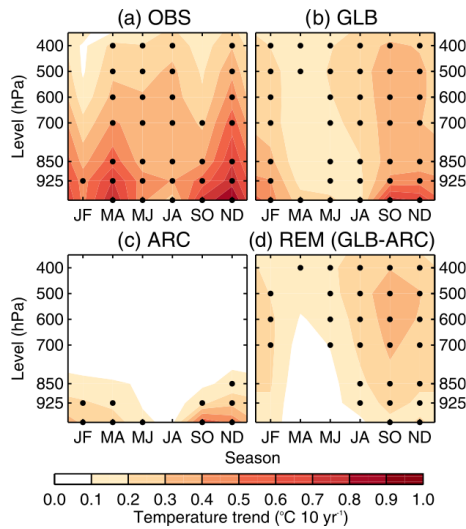
Figure 3. Local and remote drivers of Arctic warming. (a) Vertical and seasonal structure of the reanalysis ensemble-mean (OBS) Arctic-mean temperature trends (1979–2008). (b–d) As in panel (a) but for the model ensemble-mean simulations forced by observed changes in global SST and SIC (GLB), observed changes only in Arctic SIC and associated SST (ARC), and their difference (REM), respectively. Black dots show trends that are statistically significant at the 95 % level ( p < 0.05 ). These experiments enable the relative contributions of local (ARC) and remote (REM) processes to Arctic trends to be assessed, giving insight into the driving mechanisms. Source: Screen et al. (2012).
