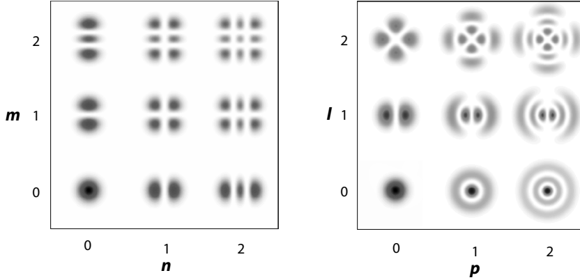
Figure 1.6.: Intensity distribution of the first few Hermite-Gauss (left) and Laguerre-Gauss (right) modes. Modified from [FS10].
