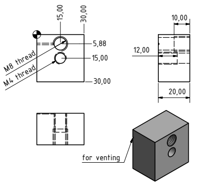
Figure D.21.: Drawing of the parts for the frames of the baffles in TCE and TCN.
