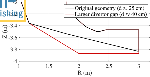
Figure 4: Comparison of the two variants of the bias electrode geometry used for the analysis in Sec. 3.
