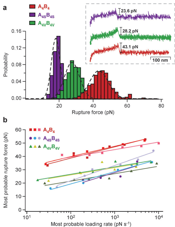
Fig. 2 Single-molecule force spectroscopy. (a) Representative rupture force histograms obtained at a retract speed of 400 nm s -1 , with n = 284 ( A_4B_4 ), n = 243 ( A_{4S}B_{4S} ) and n = 420 ( A_{4V}B_{4V} ). The dashed lines show Gaussian fits, applied to extract the most probable rupture forces. The inset shows representative force–extension curves for each CC. (b) Dynamic SMFS plot. Each CC was measured in triplicate using a different cantilever and surface (different shades of the same colour). The solid lines represent fits to the Bell–Evans model.
