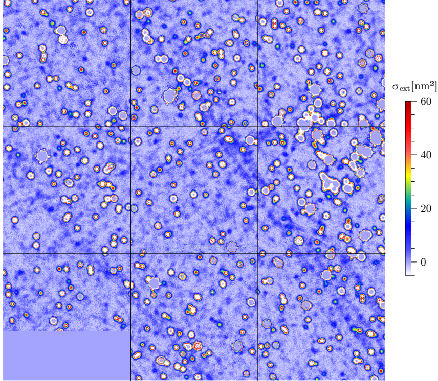
Figure 4.15: Stitched extinction cross section map of the gold nanorod sample. The map shows the average of both polarization channels. The image is composed of 9 images with a size of 100\ \mu\text{m} \times 100\ \mu\text{m} each and a pixel size of 0.25\ \mu\text{m} \times 0.25\ \mu\text{m} .
