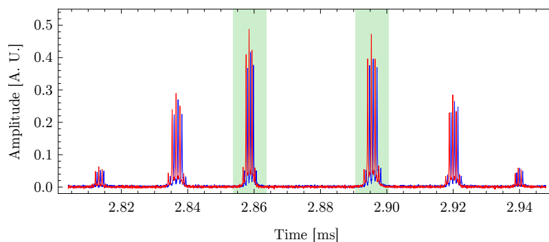
Figure 3.27: Transmission signal of the fundamental mode for both polarizations (red, blue). The two triplets of peaks within the green shaded areas are evaluated.
