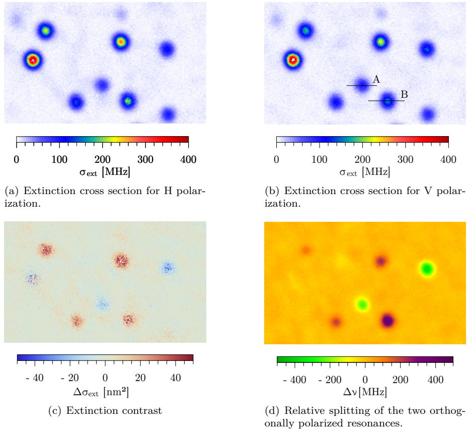
Figure 4.17: Extinction contrast and birefringence imaging of a sample with clusters of nanorods. The image size is 50 \mu\text{m} \times 30 \mu\text{m} , the pixel size is 0.2 \mu\text{m} \times 0.2 \mu\text{m} .
