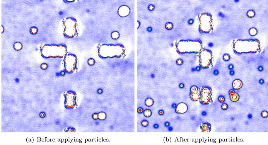
Figure 4.25: Extinction map of the sample before and after applying nanoparticles. The image size is 100\ \mu\text{m} \times 100\ \mu\text{m} , the pixel size is 0.2\ \mu\text{m} \times 0.2\ \mu\text{m} , the colour scale is the same as in figure 4.23.
