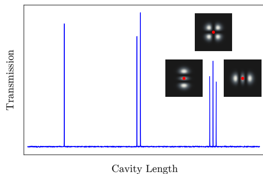
Figure 3.2: Principle of the dispersion measurement: The TEM02 and TEM20 modes are frequency shifted by a particle in the center (red dot), while the TEM11 mode stays unaffected.
