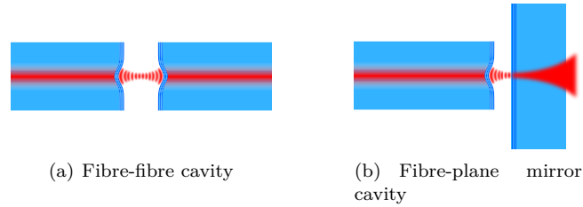
Figure 3.3: Different configurations of Fibre Fabry Pérot cavities: (a) a cavity set up of two micro machined fibres and (b) a cavity set up of a macroscopic plane mirror and a machined fibre.
