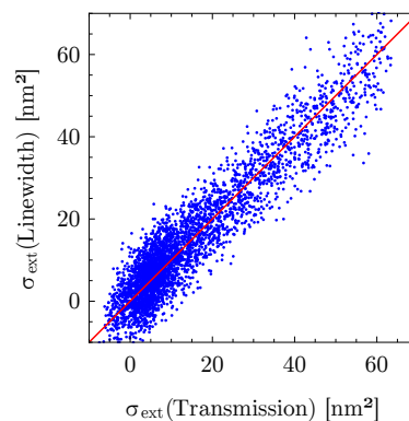
(b) Pixel-by-pixel comparison of the extinction measured by transmission or linewidth.
