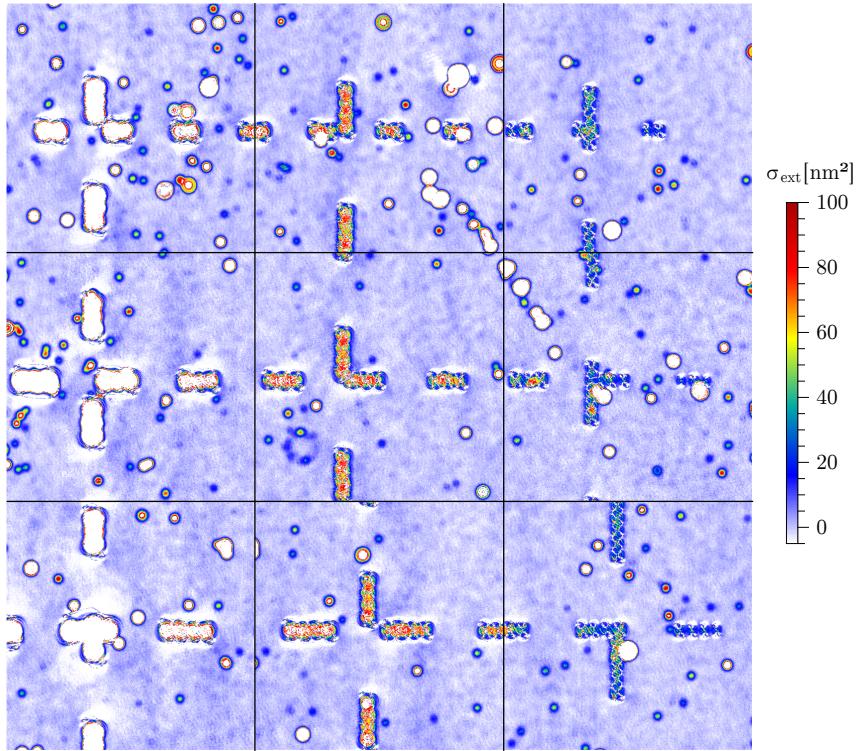
Figure 4.23: Extinction map of the sample carrying gold nanospheres of a diameter of 50 nm used for polarizability measurements. The image is composed of 9 microscope images with a size of 100\ \mu\text{m} \times 100\ \mu\text{m} with a pixel size of 0.2\ \mu\text{m} \times 0.2\ \mu\text{m} .
