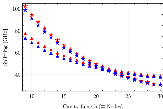
Figure 4.24: Frequency spacing between the TEM02 and TEM11 mode ( \blacktriangle ) and between the TEM20 and TEM11 mode ( \blackstar ) for H (red) and V (blue) polarization in dependence of the cavity length of fibre 16k. The values are measured without high-frequency sidebands.
