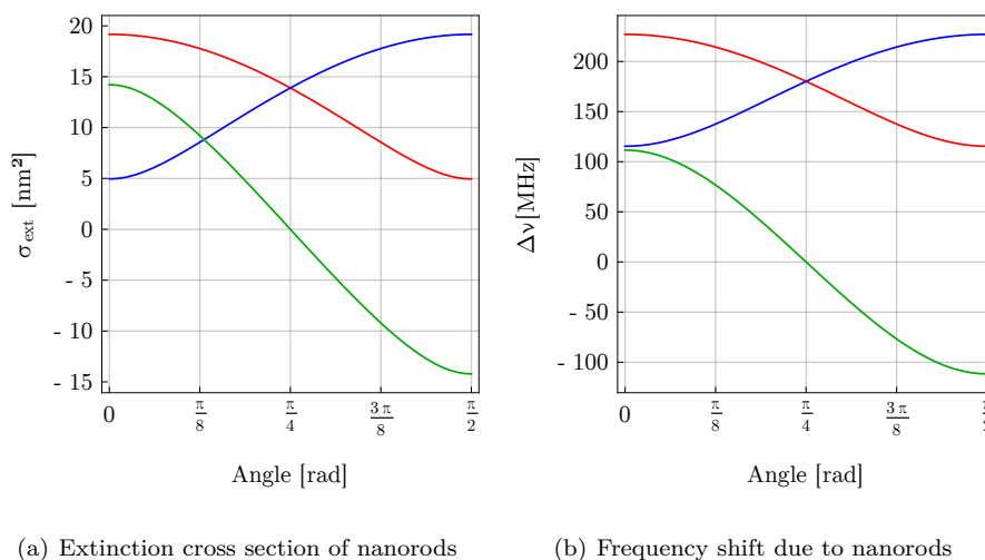
Figure 4.14: Extinction cross section and frequency shift of a cavity (wavelength 780 nm, waist 2.4 \mu\text{m} , length 32 antinodes) due to a gold nanorod (34 nm \times 25 nm \times 25 nm) depending on its orientation with respect to the H-polarisation plane of the probe light. Absolute values for polarization axes (red (H), blue (V)) and their differences (green) are calculated using numerical results for the depolarization factor [41] taking into account the shape of the particles. The values shown include effects of the surface, the particle is placed on and effects due to the small particle size.
