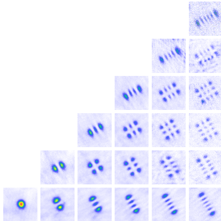
(a) Individual modes of the fundamental and the first five higher orders of transversal modes.
