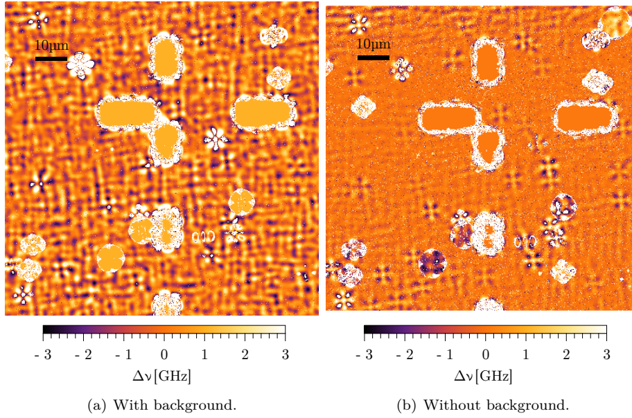
Figure 4.31: Frequency spacing map of a mirror surface carrying 50 nm gold nanospheres. The image size is 100\ \mu\text{m} \times 100\ \mu\text{m} , the pixel size is 0.2\ \mu\text{m} \times 0.2\ \mu\text{m} .
