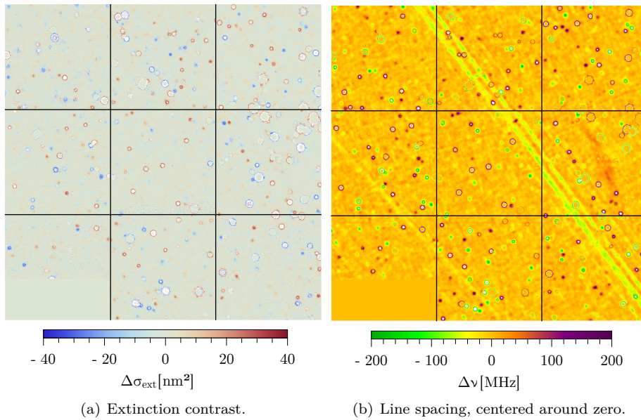
Figure 4.19: Stitched map of the extinction contrast and line spacing of the gold nanorod sample. The image is composed of 9 images with a size of 100\ \mu\text{m} \times 100\ \mu\text{m} each and a pixel size of 0.25\ \mu\text{m} \times 0.25\ \mu\text{m} .
