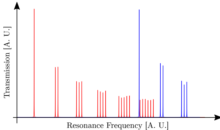
Figure 2.14: Principle of mode mixing. When the resonance frequency of a higher-order transversal mode (red) is close to the resonance frequency of a mode of the subsequent longitudinal order (blue), mode mixing can occur.
