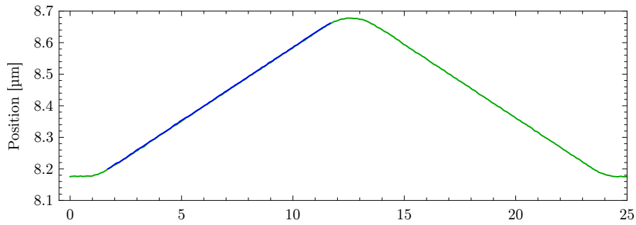
(b) Cavity length scan: movement of the positioner (green) and recorded position (blue).
