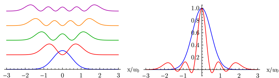
(a) Individual Hermite-Gauss modes that are added and subtracted subsequently. The offset sets are introduced for better visibility of the individual modes. (b) Sum of 4 higher order modes (red) in comparison with fundamental mode (blue)
