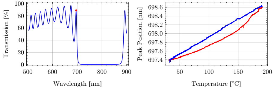
(a) Transmission spectrum of the mirror coating in the fibre measured at a macroscopic reference substrate. The first transmission maximum used for temperature measurement is marked red. (b) Shift of the first transmission peak of the mirror coating depending on the sample temperature measured at a macroscopic sample at increasing temperature (red) and decreasing temperature (blue)
