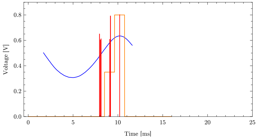
(c) Cavity transmission signals: stabilization laser ( \times 5 - 0.5 V, blue), power switching pattern (orange), probe laser (red).
