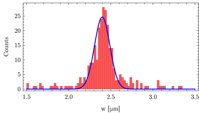
Figure 4.8: Histogram (red) and Gaussian fit (blue) of the observed particle size and thus the waist of the cavity mode.
