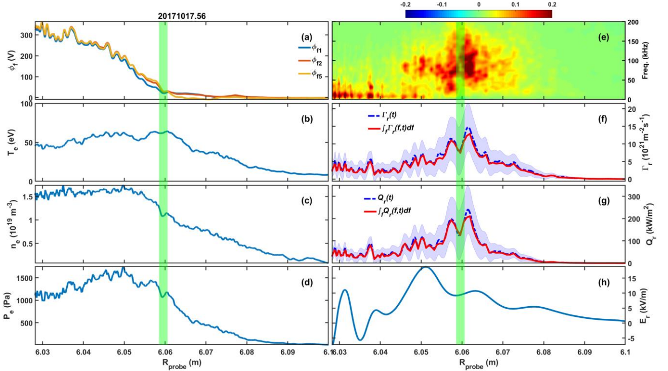
Figure 14. The radial plasma profiles, radial turbulent heat flux and particle flux of the high mirror configuration. The description is the same as Figure 7.
