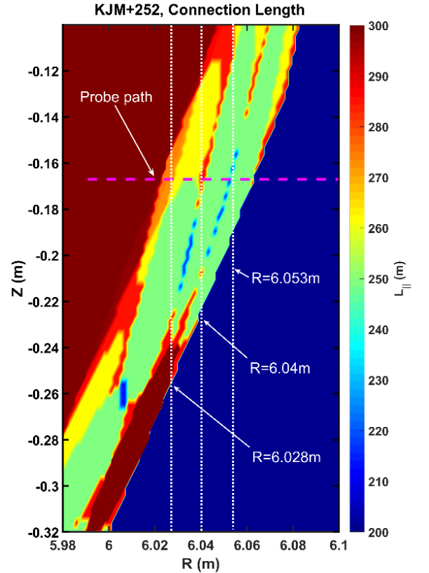
Figure 15. Two-dimensional field line connection length for the KJM+252 configuration in the poloidal plane of probe.
