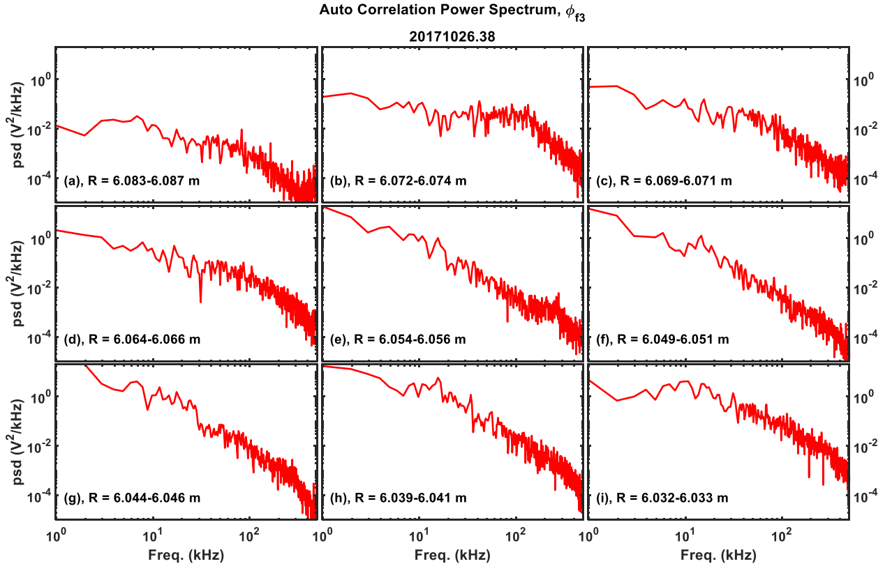
Figure 5. The auto-correlation power spectral density of floating potential \phi_{f3} at nine radial positions.
