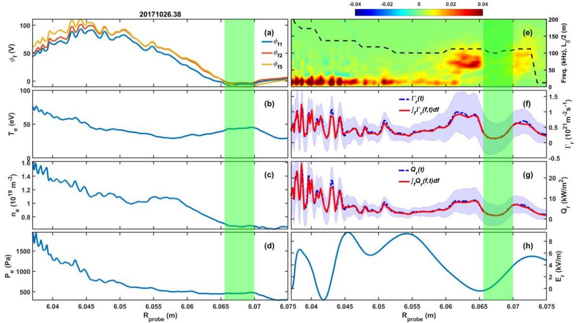
Figure 7. The turbulent radial heat flux, particle flux and plasma profiles. (a-d) floating potential, electron temperature, electron density and electron pressure. (e) The distribution of the turbulent radial particle flux in frequency space and the normalized connection length (dashed line). The green rectangle signifies a region with flat electron pressure and low radial heat flux. Positive value means the particle flux is directed outward. (f) The radial turbulent particle flux. (g) The radial turbulent heat flux. (h) Radial electric field. The shaded region in (f) and (g) denotes the standard deviation.
