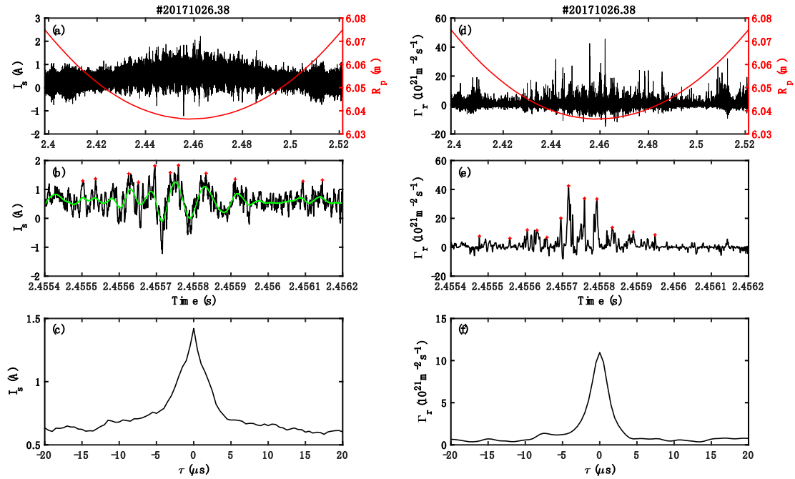
Figure 12. (a-b) Raw signal of the ion saturation current. The red crosses in (b) and (e) means that these spikes are selected by the conditional averaging procedure. The green line in (b) signifies the signal filtered by a 20 kHz low-pass filter. (c) The conditional-averaged ion saturation current in the time period of t = 2.45\text{-}2.47 s, i.e., R = 6.036\text{-}6.038 m. (d-e) Raw signal of radial turbulent particle flux. (f) The conditional-averaged radial turbulent particle flux in the same time period as (c).
