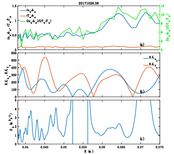
Figure 11. (a) Relative fluctuation levels of the electron density and temperature, and their ratio (\delta n_e/n_e)/(\delta T_e/T_e) . (b) Normalized gradient scale length of electron density and temperature. (c) Electron diffusion coefficient induced by turbulence.
