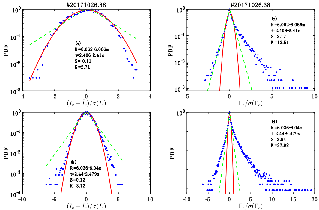
Figure 13. The probability distribution function (PDF) for the ion saturation current and the radial turbulent particle flux at two different radial positions. The skewness and kurtosis of the distribution are labelled in each panel. The red lines denote the Gaussian fitting for the PDF, and the green dashed lines denote the Laplace fitting.
