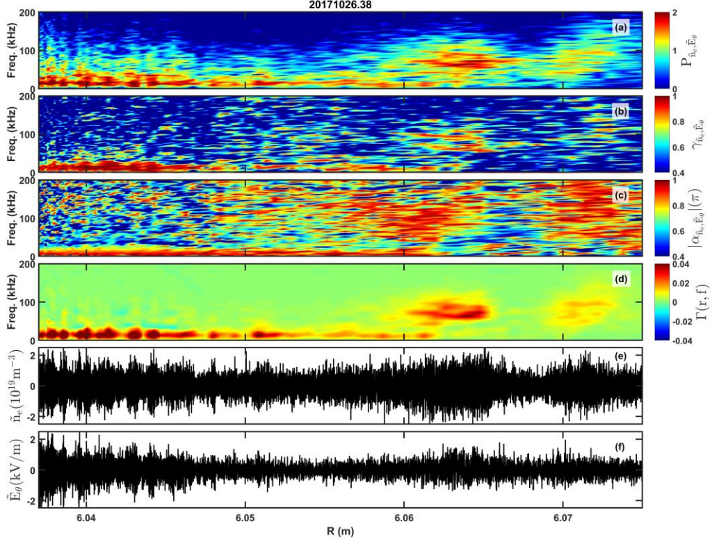
Figure 6. The cross-correlation between \tilde{n}_e and \tilde{E}_\theta . (a) Cross-correlation power spectral density P_{\tilde{n}_e \tilde{E}_\theta} ; (b) Cross-Correlation coefficient \gamma_{\tilde{n}_e \tilde{E}_\theta} ; (c) Cross-Correlation phase \alpha_{\tilde{n}_e \tilde{E}_\theta} ; (d) Turbulent particle flux.; (e) and (f) the fluctuations of n_e and E_\theta between the frequency range of 1-400 kHz, respectively.
