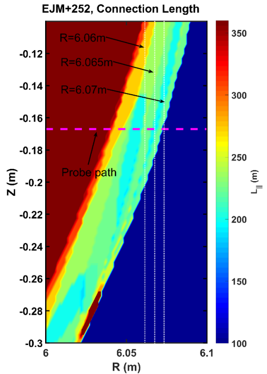
Figure 8. The two-dimension connection length on the poloidal plane of MPM for the EJM+252 configuration.
