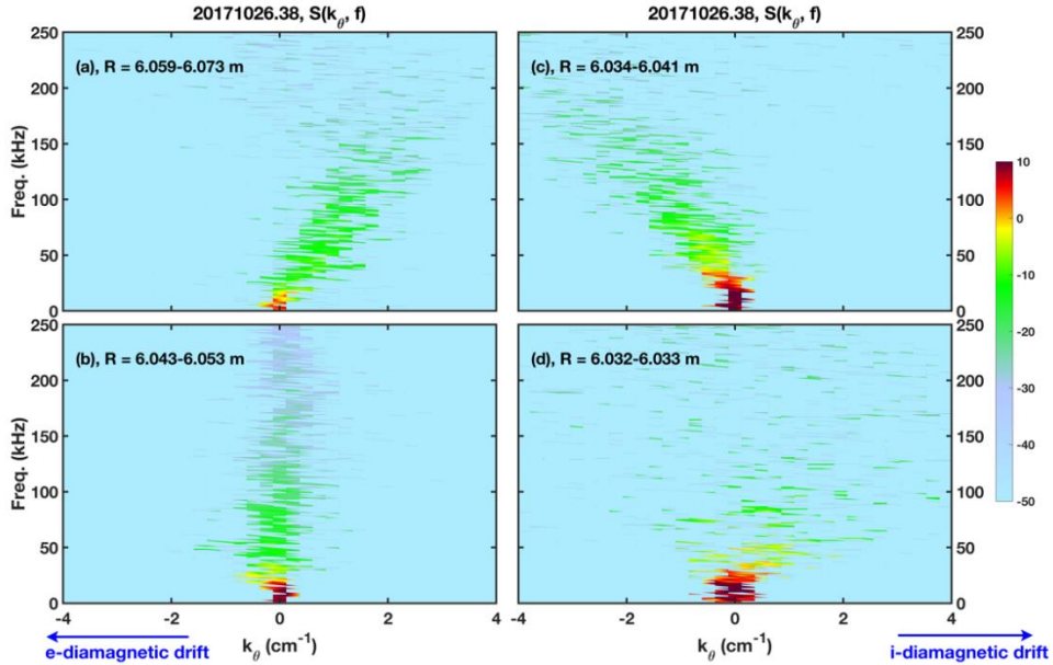
Figure 10. The poloidal cross-correlation power spectral density S(k_\theta, f) at four radial positions along the probe path for EJM+252 configuration.
