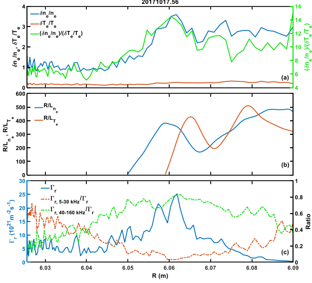
Figure 16. (a) Relative fluctuation levels of electron density and temperature. (b) Normalized gradient scale length of density and temperature. (c) Radial turbulent particle flux, the ratio of particle flux contributed by 5-30 kHz turbulence to the particle flux of the whole frequency, and the ratio of \Gamma_r from 40-160 kHz to the total particle flux.
