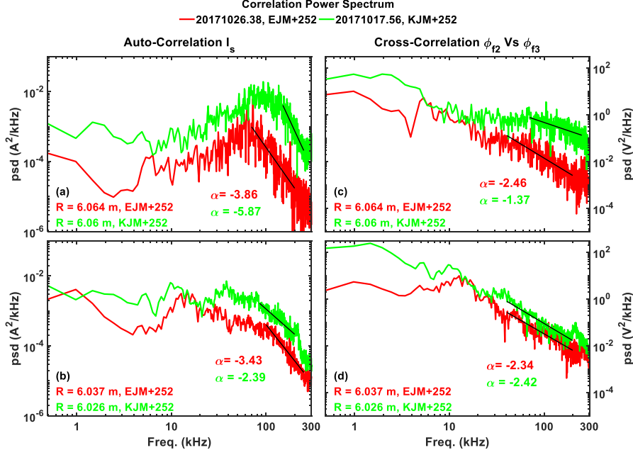
Figure 9. The APSD of the ion saturation current (left panels) and the cross-correlation spectral density (CPSD) between two radially separated floating potential pins (right panels), for both EJM+252 and KJM+252 configurations.
