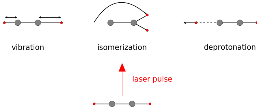
Figure 1.1: Schematic visualization of three different molecular reactions upon multi-photon-excitation by a laser pulse: vibration, isomerization, and deprotonation. The carbon atoms are depicted in grey and the hydrogen atoms in red.
