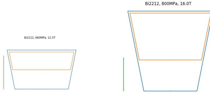
Figure 3 - Impact of the peak field in the TF conductor on radial build and machine sizing, from the systems code PROCESS (see text).
