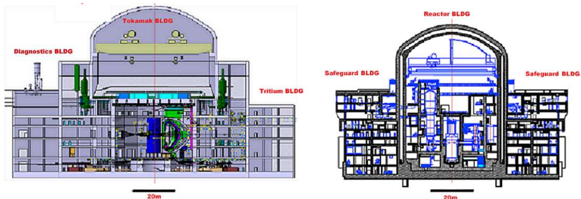
Figure 7 - DEMO Tokamak Building Complex (compared with EPR)
