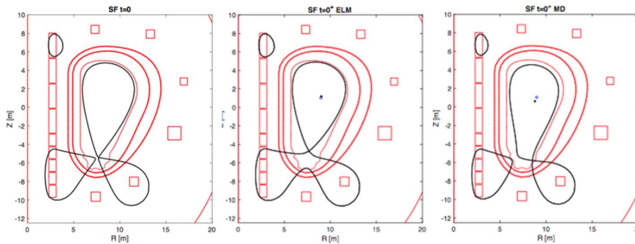
Figure 6 - Simulations of SF limb positions in normal equilibrium (left), following an ELM (middle), and following a vertical displacement (right). In each of the two disturbed cases, the limb positions and relative power-sharing are substantially altered and risk placing high power densities on unprotected in-vessel components. [2829]
