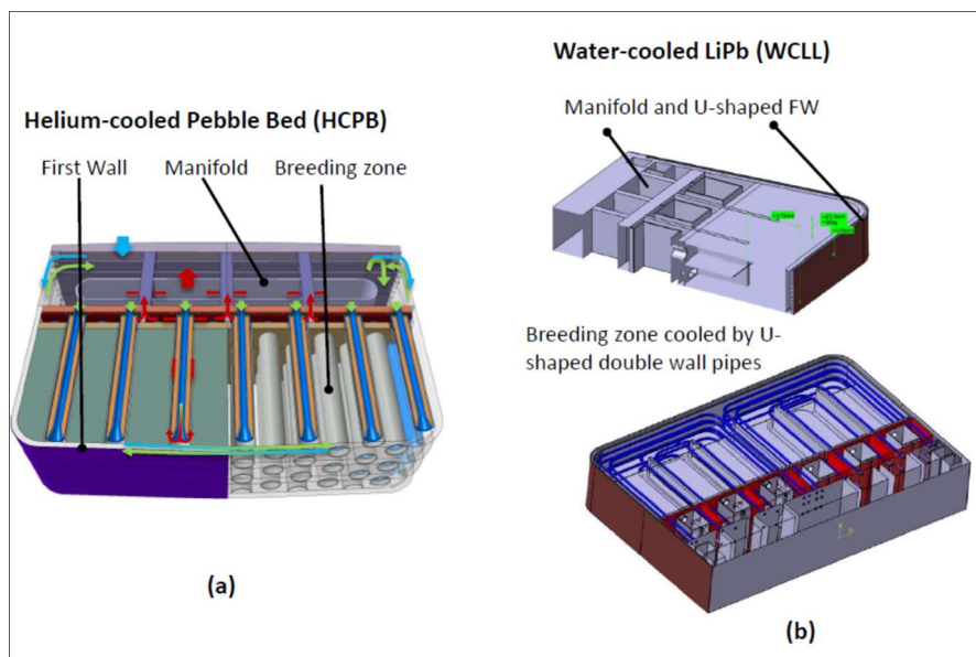
Figure 9 - Schematic representations of (a) HCPB and (b) WCLL breeding blanket concepts.
