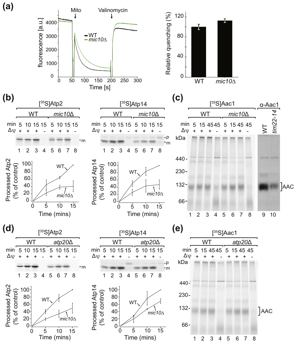
Fig. 4. MICOS is required for efficient import of TIM23 pathway substrates. (a) Mitochondrial membrane potential ( \Delta\psi ) was measured in wild-type and mic10 \Delta yeast using the potential sensitive dye 3,3'-dipropylthiadicarocyanine iodide (DiSC 3 ) and monitoring of fluorescence. Relative fluorophore quenching, used to calculate \Delta\psi , is shown in the adjacent bar graph (mean \pm SEM, n = 3). (b) Radiolabeled Atp2 and Atp14 were imported into isolated mitochondria from wild-type and mic10 \Delta cells. Mitochondria were treated with proteinase K and samples analyzed by SDS-PAGE and digital autoradiography. Import of wild-type at the longest time point was set to 100% (mean \pm SEM, n = 3). (c) Radiolabeled Aac1 was imported into isolated wild-type and mic10 \Delta mitochondria. Samples were solubilized, resolved by BN-PAGE and analyzed by digital autoradiography. A BN-PAGE analysis of the mature AAC complex in wild-type and tim22-14 [51] using Aac1 antibody is shown alongside to show the running behavior of AAC at steady state. (d) Radiolabeled Atp2 and Atp14 were imported into isolated mitochondria from wild-type and atp20 \Delta and samples analyzed by SDS-PAGE and digital autoradiography. Import of wild-type at the longest time point was set to 100% (mean \pm SEM, n = 3). Quantifications from three separate experiments are shown. (e) Radiolabeled Aac1 was imported into isolated wild-type and mic10 \Delta mitochondria. Samples were solubilized in digitonin, resolved by BN-PAGE analysis and analyzed by digital autoradiography. P, precursor; m, mature.
