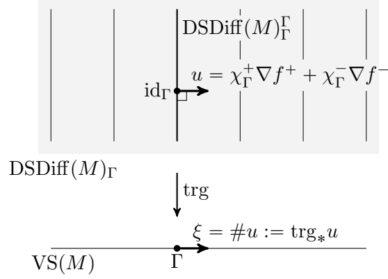
Figure 2: Riemannian submersion for the groupoid. Here \text{DSDiff}(M)_\Gamma^\Gamma is the group of discontinuous diffeomorphisms \text{SDiff}(D_\Gamma^+) \times \text{SDiff}(D_\Gamma^-) , and u is a horizontal vector field projecting to \xi = \#u . The latter can be regarded as the velocity of the vortex sheet \Gamma , and \langle \xi, \xi \rangle_{\text{VS}} = \langle u, u \rangle_{L^2} .
