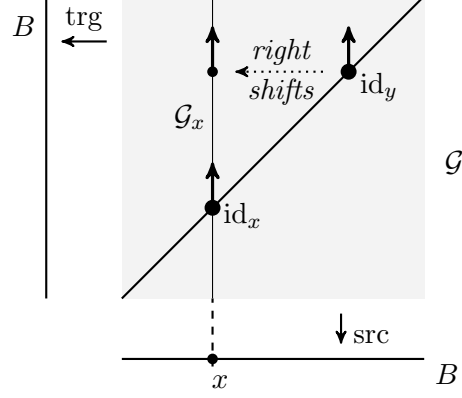
Figure 5: A transitive groupoid \mathcal{G} \rightrightarrows B is depicted as a square. The vertical projection is the source map \text{src}: \mathcal{G} \rightarrow B , the horizontal projection is the target map \text{trg}: \mathcal{G} \rightarrow B , while horizontal arrows are right translations. A section of the algebroid is a collection of vertical vectors attached to the diagonal \text{src} = \text{trg} .
