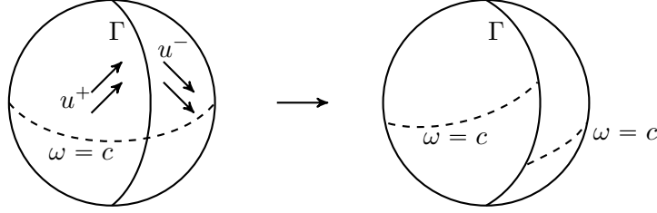
Figure 4: Smooth levels of the vorticity \omega on a sphere are transported by the flow with velocity u^\pm and hence getting broken along the vortex sheet \Gamma .
