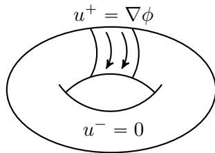
Figure 6: An irrotational steady solution with a vortex sheet. This solution delivers the global maximum of the corresponding potential \mathcal{P} on \text{VS}(M) .
