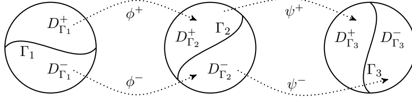
Figure 1: Elements of the groupoid \text{DSDiff}(M) and their composition rule.
