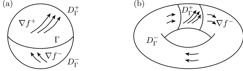
Figure 3: (a) Pure vortex sheet solutions on a sphere. Their motion is a geodesic on \text{VS}(S^2) . (b) Irrotational, but not pure, vortex sheet solutions. Their motion can be viewed as a trajectory of a Newtonian system in a magnetic field on \text{VS}(T^2) .
