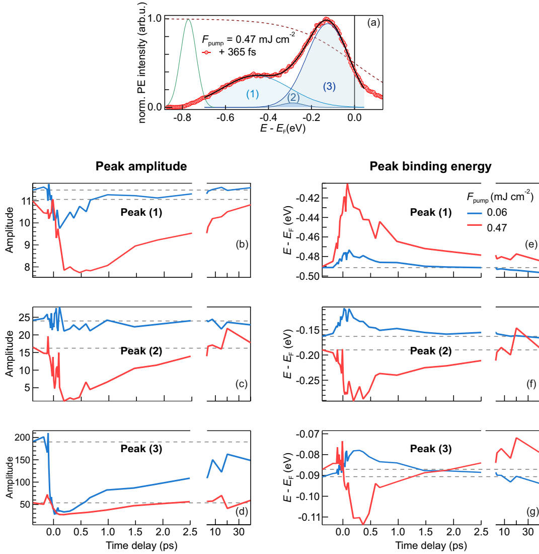
FIGURE B.1: (a) EDC at \Gamma , 365 fs after photoexcitation with 0.47 \text{ mJ cm}^{-2} and at 110 K (solid red). The fit curve (black line) is composed of three Gaussian peaks (blue shades) multiplied by a FDD distribution (red dashed curve), and convolved with a Gaussian accounting for the energy resolution (green curve). (b) - (g) Best-fit parameters of the peak amplitude and binding energy relative to E_F for two data set at low (blue) and high (red) fluence, respectively. See text for details.
