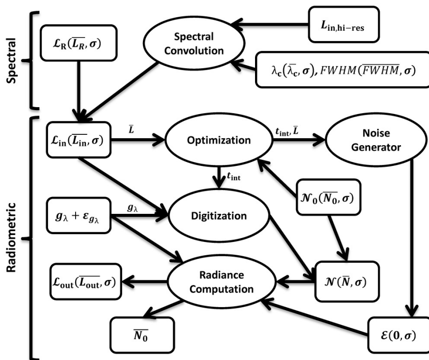
Figure A1. Scheme of operation of the sensor simulator.
