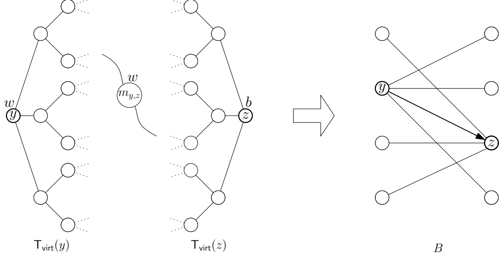
Figure 3: In this example, the merged node of T_{\text{virt}}(y) and T_{\text{virt}}(z) has the same color as node y , hence the edge \{y, z\} in B is oriented from y to z .
