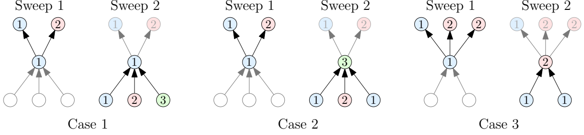
Figure 1: Examples of the output of the 3-partial 3-coloring algorithm, running at the central node v , in a graph where the degree is 5. The figure shows 3 cases: v keeps the color chosen during the first sweep, v switches to the special color in the second sweep, v switches to color 2 in the second sweep.
