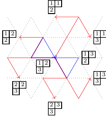
FIGURE 1. Semistandard tableaux of shape \lambda = (2, 1) and their paths, for \mathfrak{sl}(3, \mathbb{C}) .
