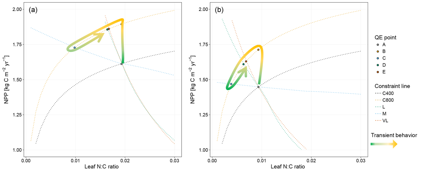
Figure 1. Graphic expression of the baseline quasi-equilibrium framework in understanding plant production response to elevated CO 2 based on photosynthetic (C400, C800 refer to CO 2 = 400 and 800 ppm, respectively) and nitrogen cycling constraints in the medium (M), long (L), and very long (VL) terms under the assumption of a (a) variable wood N : C ratio and a (b) fixed wood N : C ratio. The photosynthetic constraint is an analytical expression of the Farquhar leaf photosynthesis model that relates leaf chemistry (i.e., N : C ratio) to production, simplifying leaf to canopy scaling. The nutrient recycling constraint is an analytical expression of the soil nutrient downregulation effect on production, assuming soil organic matter structures as in Fig. 2. The quasi-equilibrium points at various timescales (A, C, D, and E) were calculated by solving for the intersection of the photosynthetic and nutrient cycling constraints through the two-timing approximation. Initially the system is in equilibrium between photosynthetic N demand and soil N supply at CO 2 = 400 ppm (A). The instantaneous response to a doubling of CO 2 is a sharp increase in production at a constant leaf N concentration (B). Under nutrient-limited conditions, the soil N supply cannot sustain this increase in production over time. A negative feedback moves the quasi-equilibrium point towards point C, where the M-term pools equilibrate with eCO 2 . The system gradually moves toward point D and E as the L and VL pools equilibrate. The downward slopes of the N recycling constraint curves with an increasing leaf N : C ratio are due to the increased proportional loss of mineralized N through leaching as the rate of N cycling increases with leaf N concentration.
