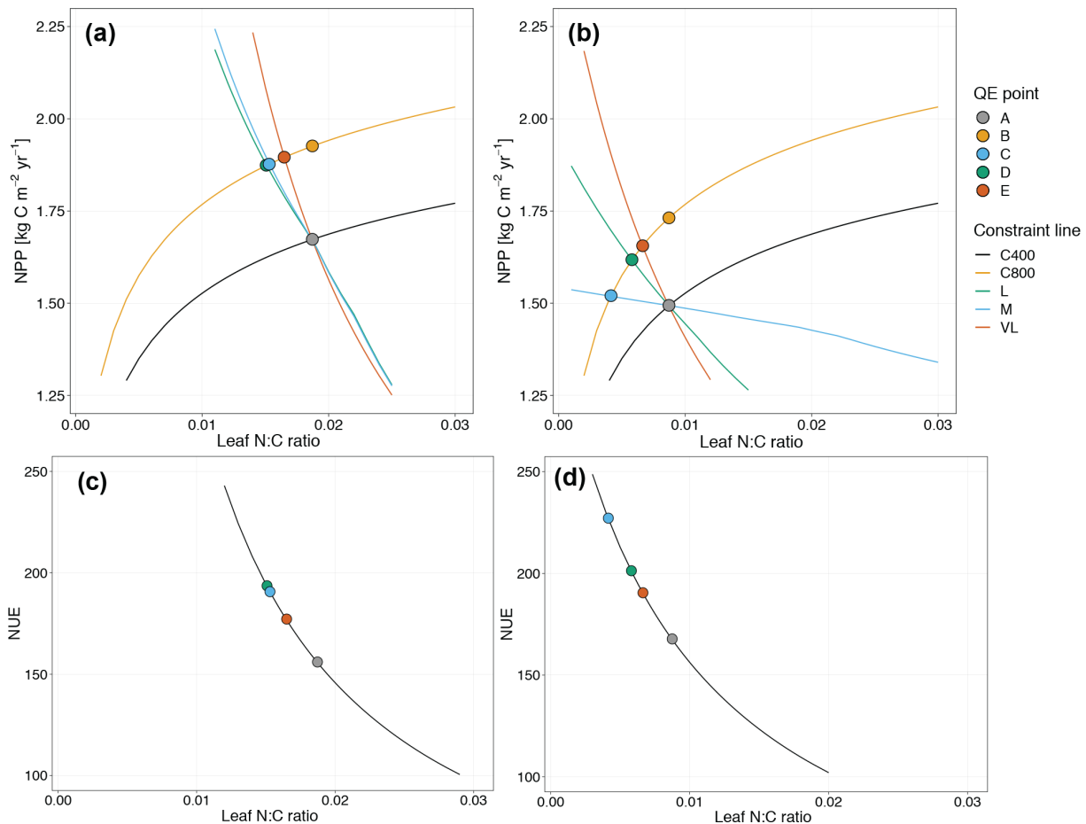
Figure 6. Graphic interpretation of the priming effect on plant net primary production ( a , b ) and nitrogen use efficiency ( c , d ) response to CO 2 fertilization under variable wood N : C ratio ( a , c ) and fixed wood N : C ratio assumptions ( b , d ). Constraint lines C400, C800, M, L, and VL refer to photosynthetic constraints at CO 2 = 400 ppm, CO 2 = 800 ppm, medium-term, long-term, and very-long-term nutrient recycling constraints, respectively. Point A is the quasi-equilibrium point at CO 2 = 400 ppm, point B is the instantaneous response point at elevated CO 2 , and points C, D, and E are the M-, L-, and VL-term equilibrium points at elevated CO 2 .
