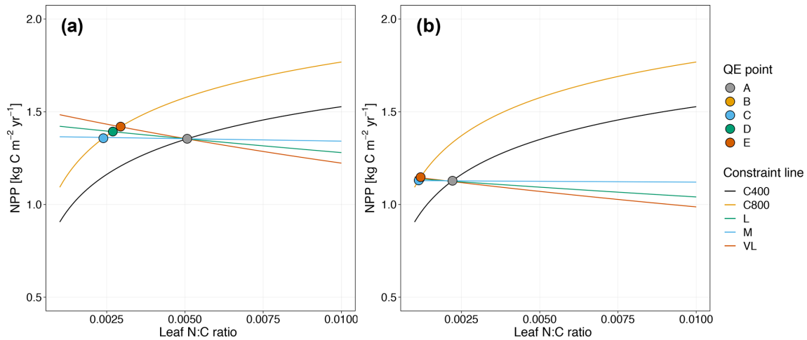
Figure 5. Graphic interpretation of the effect on CO 2 responses with models incorporating the relative demand assumption based on variable (a) and fixed (b) wood N : C ratio assumptions. Constraint lines C400, C800, M, L, and VL refer to photosynthetic constraints at CO 2 = 400 ppm, CO 2 = 800 ppm, medium-term, long-term, and very-long-term nutrient recycling constraints, respectively. Point A is the quasi-equilibrium point at CO 2 = 400 ppm, point B is the instantaneous response point at elevated CO 2 , and points C, D, and E are the M-, L-, and VL-term equilibrium points at elevated CO 2 .
