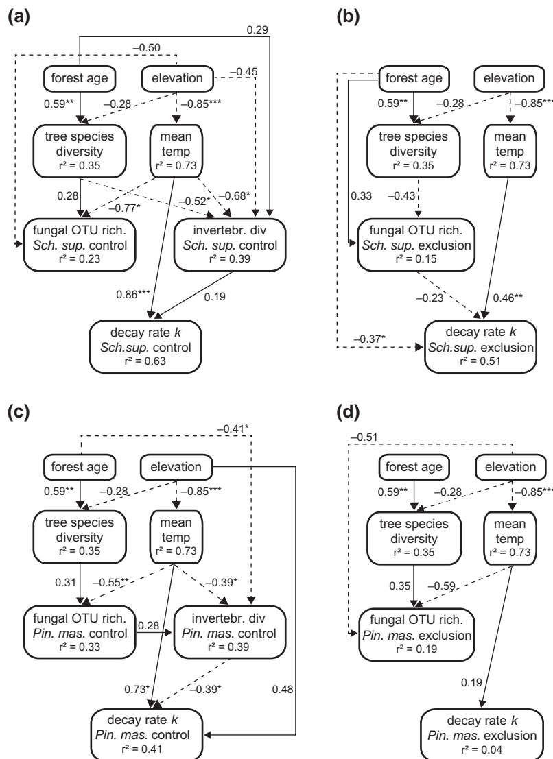
Figure 3. Structural equation models for both species and treatments. (a) S. superba control treatment, Fisher's C = 8.33 , p = 0.99 ; (b) S. superba exclusion treatment, Fisher's C = 11.86 , p = 0.75 ; (c) P. massoniana control treatment, Fisher's C = 13.06 , p = 0.79 ; (d) P. massoniana exclusion treatment, Fisher's C = 9.91 , p = 0.97 . Solid lines represent positive relationships, dotted lines negative. Standardized path coefficients and significance levels are shown for each pair of connected variables; *** p < 0.001 , ** p < 0.01 , * p < 0.5 . temp = temperature, fungal OTU rich. = fungal OTU richness, invertebr. div = macro-invertebrate diversity, Sch. Sup. = Schima superba , Pin. mas. = Pinus massoniana . Detailed model results are given in the Supplementary material Appendix 3 Table A1.
