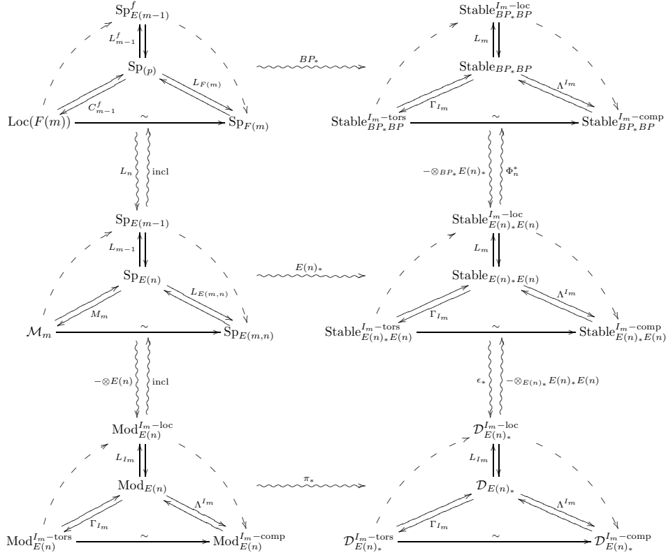
FIGURE 1. Topological and algebraic local duality contexts.
