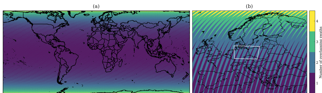
Figure 2. Spatial coverage of one CO 2 M satellite within its 11 d repeat cycle (a) globally and (b) over Europe. The white square marks the COSMO-GHG model domain in which the number of overpasses is either one or two. The exact locations of the stripes are arbitrary and depend on the Equator starting longitude (here: 0° E) of the satellite.
