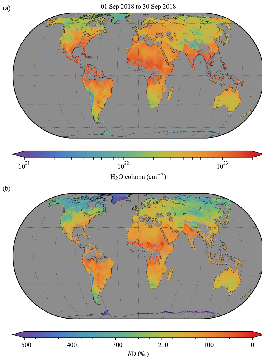
Figure 10. Global plots of H 2 O (a) and δD (b) averaged over September 2018 on a 0.5° × 0.5° grid. The average of δD is weighted with the H 2 O column for mass conservation purposes.
