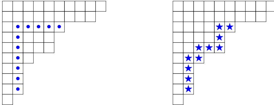
FIGURE 2.1. An 11-hook (left) and the corresponding 11-rim hook (right).
