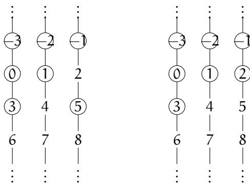
FIGURE 4.1. An abacus for \lambda = (2, 1) on the left, and an abacus for \lambda = (0, 0) on the right.
