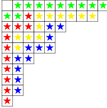
FIGURE 2.2. The 11-core for (10, 9, 6, 5, 5, 3, 2, 2, 2, 1) is the partition (1) .
