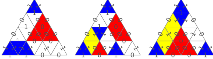
FIGURE 2.3. Puzzles for computing products in H_T^*(\text{Gr}(2,4))
