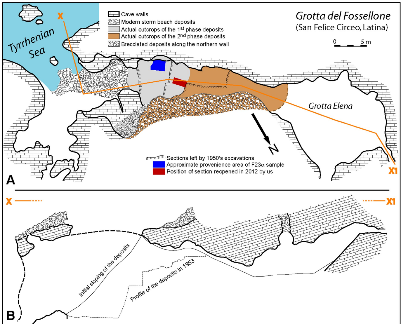
Fig 2. Plan and section of Grotta del Fossellone. (A) Plan of the cave with location of the 2012 fieldwork, intact remnants of Pleistocene deposits and approximate provenience of F23α sample from the 1947–1953 excavation. Modified from [50]. (B) Schematic longitudinal section of the cave showing the large opening in the roof, modified from [49]. Courtesy of the Istituto Italiano di Paleontologia Umana.
