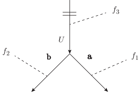
FIGURE 5.1. The partition function with a single-brane insertion that has an open-string modulus U and framing factor f_3 , and two brane stacks that have open-string moduli \mathbf{a} = (a_1, a_2, \dots) , \mathbf{b} = (b_1, b_2, \dots) and framing factors (f_1, f_2) . By the inverse arrow in the preferred leg we assign the transpose Y'_3 of the Young diagram Y_3 , where we note the relation \mathcal{R}_{Y_1 Y_2 Y'_3}(x, x) = \mathcal{C}_{Y_1 Y_2 Y'_3}(x) in (3.5).
