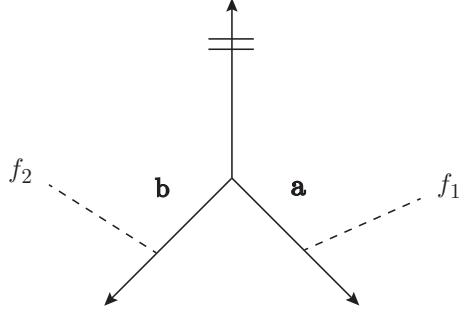
FIGURE 4.1. The vertex with two brane stacks with open-string moduli \mathbf{a} = (a_I)_{I=1,2,\dots} , \mathbf{b} = (b_I)_{I=1,2,\dots} and framing factors f_1 and f_2 .
