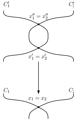
FIGURE 1. \Delta_{g_1:g_2}
