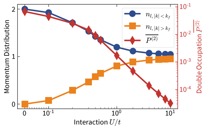
FIG. 6. (Color online) Partially integrated momentum-distribution function and real-space double occupation for \rho = 1/3 . We show data for superlattice amplitude V/t = 3 and phase \delta = \pi/3 . \overline{P^{(2)}} is the double occupation averaged over one superlattice cell. Increasing the strength U of the interaction suppresses double occupation for the MI phase. In momentum space, all particles remain in the lowest band, but, as U increases, states below and above the Fermi wavenumber k_F become evenly occupied. The lines are guides to the eye.
