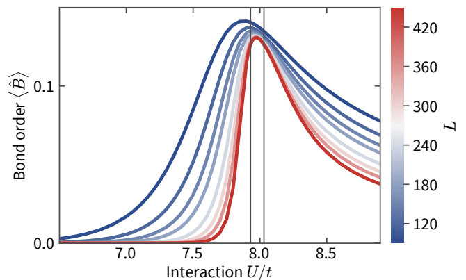
FIG. 10. Bond-order parameter across the BI-SDI-CI transition. At \delta = \pi/3 , the system is as depicted in Fig. 2, i.e., the potential energies on sites 1 and 3 are degenerate, and site 2 is lower in energy. Data were computed for open boundaries without inversion symmetry for L \in \{90, 120, 150, 180, 240, 300, 360, 450\} . The vertical lines indicate the two phase transitions, as determined from the gap data shown in Fig. 11.
