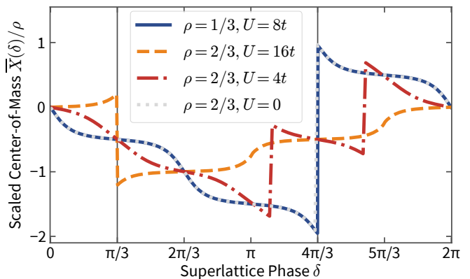
FIG. 13. Center-of-mass motion . Scaled center-of-mass of an open system as a function of superlattice phase \delta . For every cycle of \delta \rightarrow \delta + 2\pi , there are discontinuities corresponding to minus the Chern number of the respective phase. The center-of-mass coordinate \bar{X} [see Eq. (16)] is divided by particle density \rho to show that the results for the Mott-insulating phase at \rho = 1/3 agree with the behavior of the noninteracting phase for \rho = 2/3 . Data were obtained for length L = 60 .
