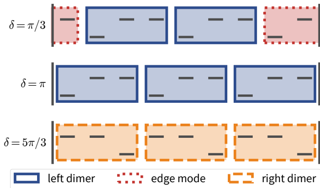
FIG. 9. (Color online) Lattice configurations for open boundary conditions. Different choices of \delta change the boundary conditions. These boundary conditions determine edge-state properties of the groundstate of the SDI phase: The two asymmetric lattice configurations, \delta = \pi and \delta = 5\pi/3 , support left and right dimerized groundstates, respectively. However, for \delta = \pi/3 , the symmetric lattice configurations support neither groundstate, leading to the existence of gapless edge modes.
