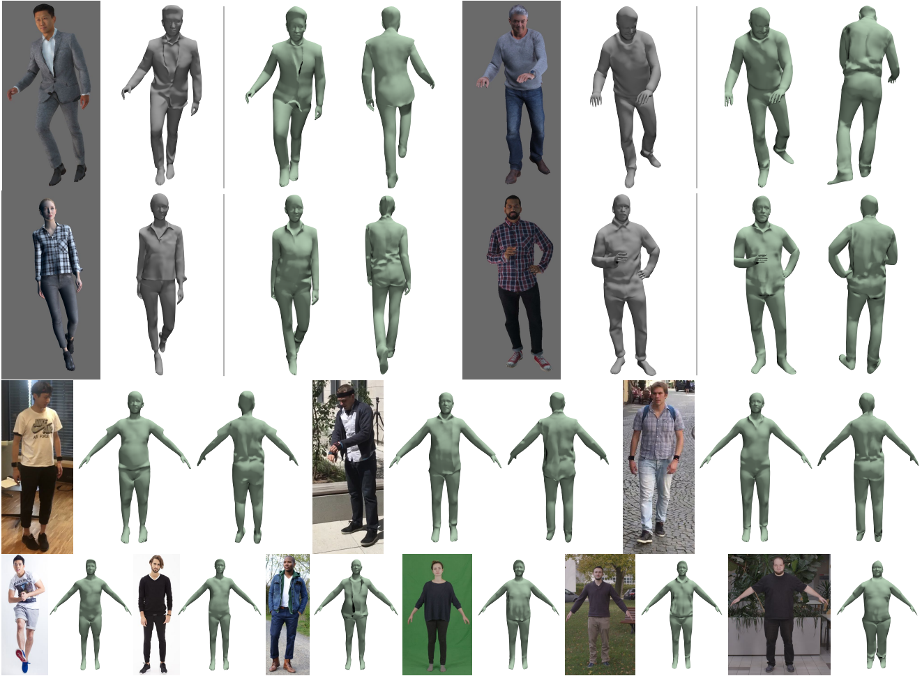
Figure 5. Our 3D reconstruction results (green) on four different datasets. We compare against ground truth (grey) on our synthetic dataset (rows 1 and 2). Qualitative results on 3DPW (3rd row), DeepFashion (4th row left) and PeopleSnapshot (4th row right) demonstrate, that our model generalizes well to real-world footage. Details on the back of the models are hallucinated by our model.
