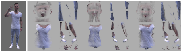
Figure 8. Partial textures computed with different methods. From left to right: Input, ground truth UV mapping, DensePose, HMR.
