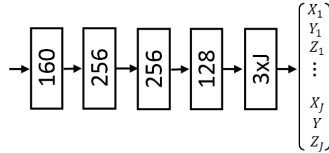
Fig. 5. Lightweight fully connected network that forms Stage II of our pipeline. The network ‘lifts’ inferred 2D body pose, augmented with joint detection confidences and 3D pose encodings to root-relative full body 3D pose (X_j, Y_j, Z_j) , leveraging full body context to fill in occluded joints .
