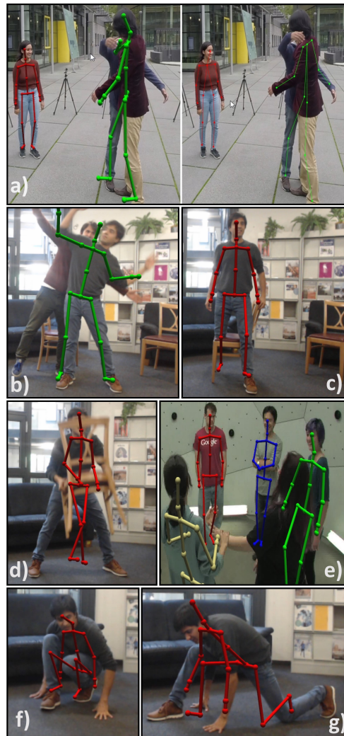
Fig. 14. Failure Cases: a),c) 3D pose inaccuracy due to 2D pose limb confusion, b) Person not detected due to neck occlusion, d),e) 3D misprediction and person undetected under extreme occlusion, f),g) 2D-3D pose alignment becomes unreliable in cases with significant self occlusion
