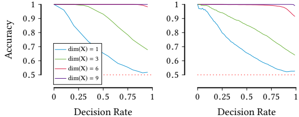
Figure 1: [Higher is better] Accuracy over top- k % pairs sorted by confidence, for different generating models of X, Y , and different dimensionality of X , with \dim(Z) = 3 fixed. The baseline is at 0.5. On the left, X, Z and W are \sim \text{Normal}(0, 1) , while on the right, we consider the adversarial case where we use out-of-model source distributions.
