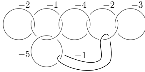
FIGURE 2. An integral surgery from \Sigma(2, 5, 17) to Y .
