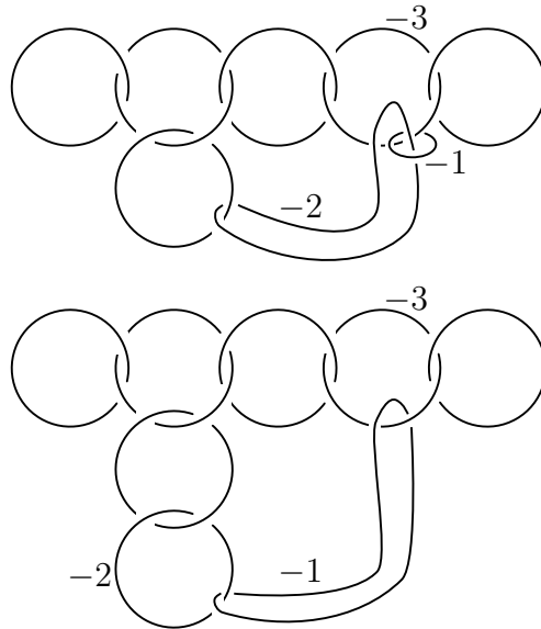
FIGURE 4. Blowing up in the diagram.
