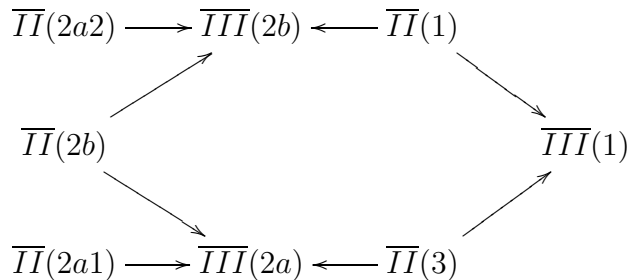
FIGURE 1. Incidence relations among the boundary components of the compactification of \mathcal{M}_0^* in \overline{\mathcal{M}}^* . We denote A \rightarrow B when the boundary component B is contained in the closure of the boundary component A .
