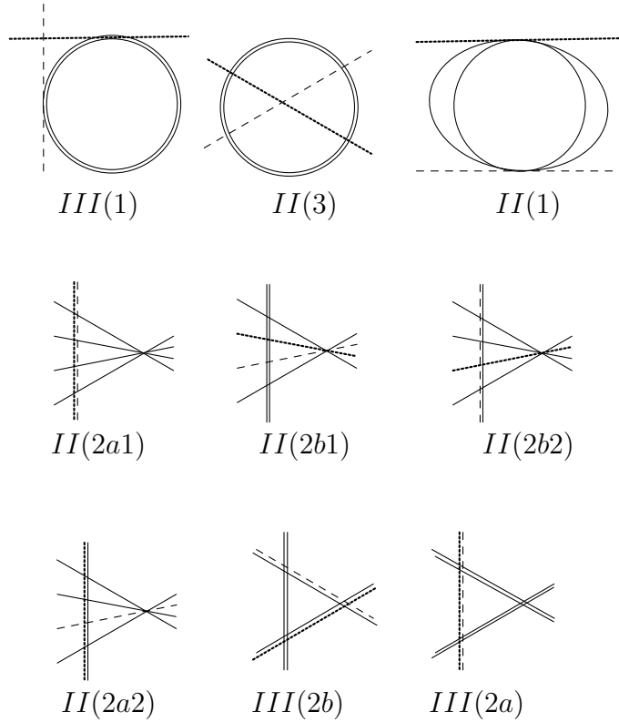
FIGURE 2. Triples parametrized by \overline{\mathcal{M}}(1,1) \setminus \mathcal{M}_0 . The dotted and dashed lines represent the lines L_1 and L_2 , respectively (see Lemma 2.15).
