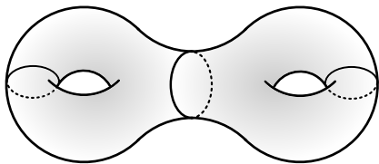
Figure 1: A genus-2 Riemann surface can be decomposed into two pairs of pants.
