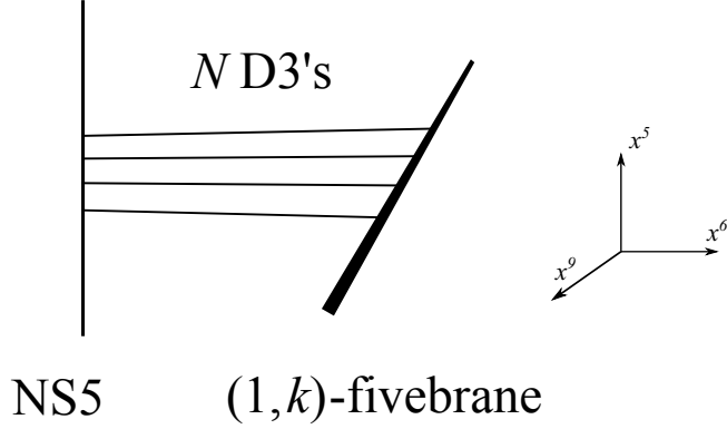
Figure 4: The NS5-D3-(1, k ) brane system in type IIB string theory.
