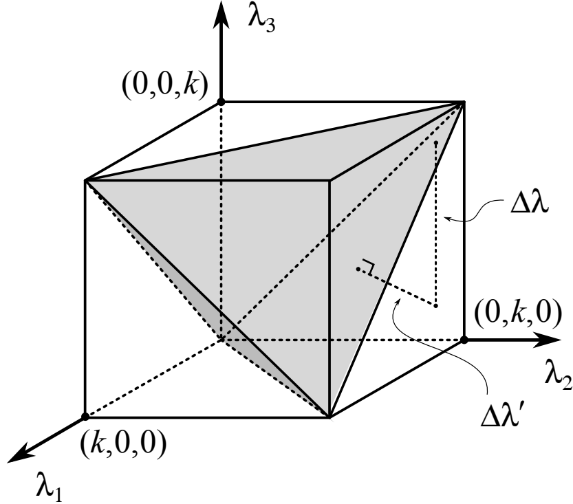
Figure 7: The definition of \Delta\lambda and \Delta\lambda' = \Delta\lambda/\sqrt{3} .
