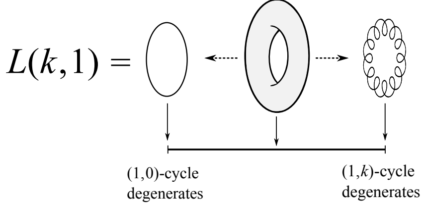
Figure 3: The Lens space L(k, 1) can be viewed as the total space of a 2-torus fibered over an interval. Near each endpoint of the interval, a particular cycle of the torus degenerates.
