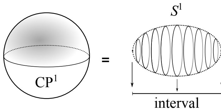
Figure 2: \mathbb{C}\mathbb{P}^1 can be viewed as the total space of a circle fibration over an interval, with degenerate fibers at the endpoints of the interval.
