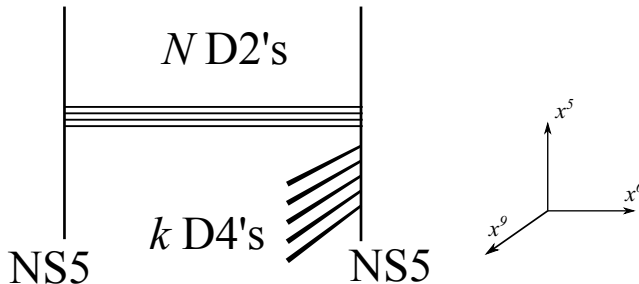
Figure 6: The NS5-D2-NS5-D4 brane system in Type IIA string theory obtained by dimensionally reducing the system in figure 4.
