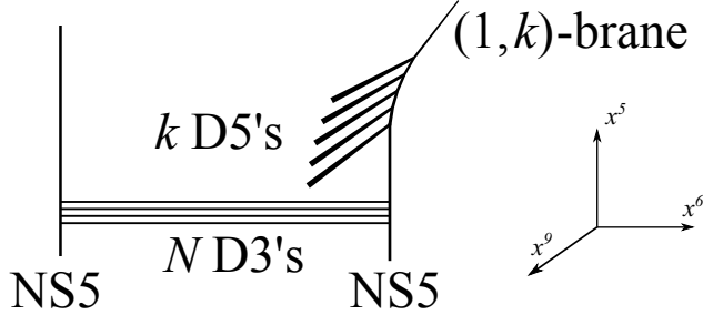
Figure 5: The (1, k) -brane in figure 4 is a bound state of an NS5-brane and k D5-branes.
