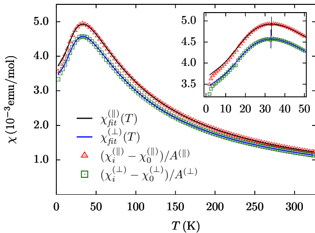
FIG. 3. Static susceptibilities of CPB for two orientations of the small magnetic field of 0.1 T ( \parallel and \perp to the c axis) as functions of temperature. Open symbols indicate measured data (minus offsets and divided by geometry factors, see Eqs. (6)). For the sake of clarity, only every sixth of these data points is plotted in the main plot and every second point in the inset. Solid lines show the best fit \chi_{fit}^{(\parallel,\perp)}(T) = \chi^{(0)}(T) + \chi_{corr}^{(\parallel,\perp)}(T) , corresponding to J/k_B = 52.0 K and \delta = -0.019 (see text). The excellent match between calculated and measured data is emphasized in the inset. Vertical lines indicate the positions of the Bonner-Fisher maxima. The difference in height can be mainly attributed to the g -factors of the two field directions.
