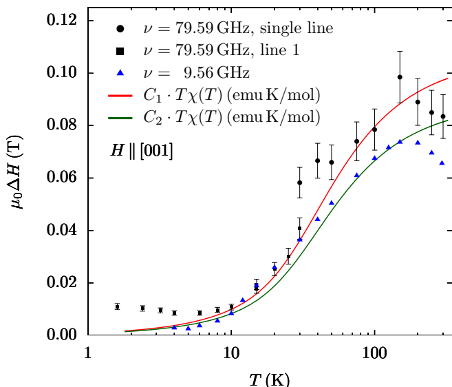
FIG. 9. Linewidth for CPB as a function of temperature at 9.56 GHz and 79.59 GHz with the field applied along the c axis. For comparison, the curves C_{1,2}T\chi(T) with the static susceptibility \chi of the isotropic Heisenberg chain and with C_1 = 0.25 T mol/(emu K), C_2 = 0.2 T mol/(emu K) are shown.
