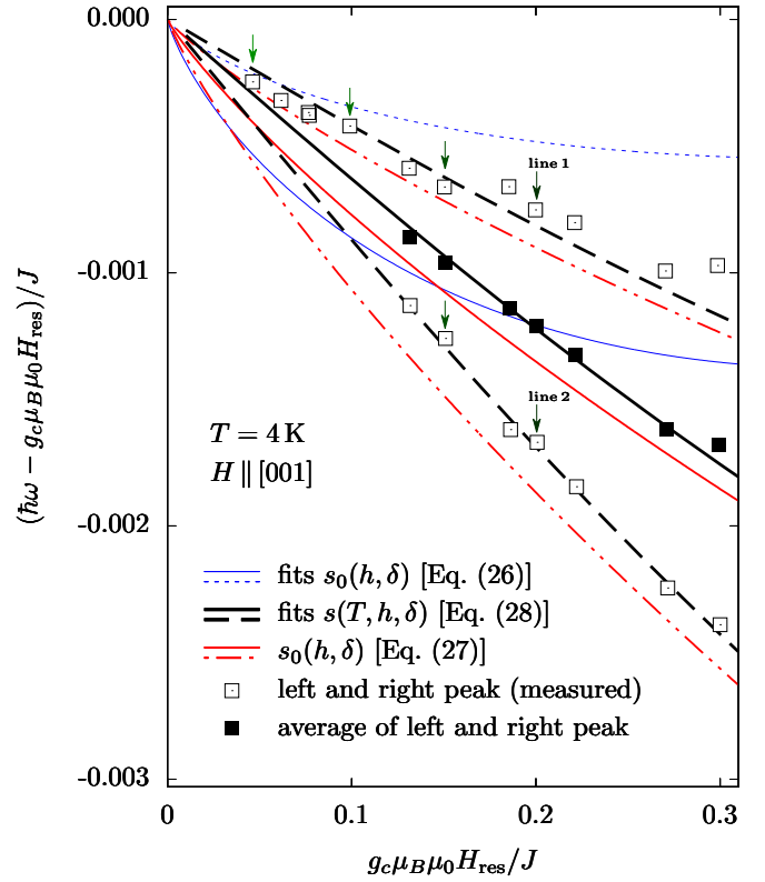
FIG. 7. Resonance shift for CPB at 4 K with magnetic field oriented along the c axis, calculated from resonance positions presented in Fig. 6. Experimental data (squares) are compared with different theoretical predictions (solid lines for the averaged shift, dashed lines for the shifts of line 1 and line 2). Frequencies and resonance fields are rendered dimensionless by multiplying with \hbar/J and g_c \mu_B \mu_0/J (with temperature independent g_c = 2.153 ; see Sec. VB 1). Arrows indicate the shifts of the exemplary spectra shown in the inset of Fig. 6.
