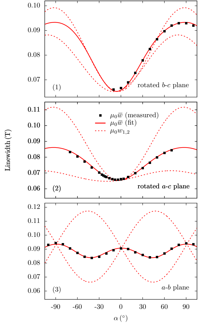
FIG. 5. Angular dependence of the measured ESR linewidth for CPB (dots) at frequency \nu = 9.56 GHz and at room temperature for rotation of the magnetic field in planes containing the c axis (top and middle) and in the a' - b plane (bottom), compared to the fitted theoretical curves \mu_0\bar{w} (solid lines). Dashed lines indicate the linewidths \mu_0w_1 and \mu_0w_2 of the two individual, unresolved lines (see Eq. (14) and text).
