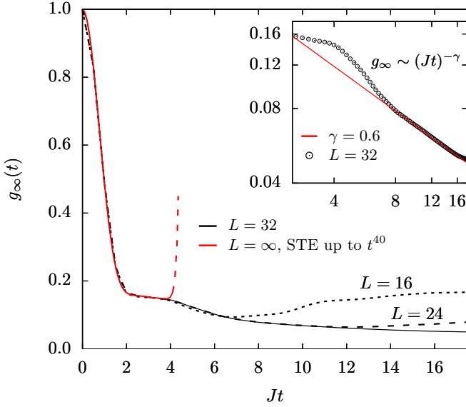
FIG. 12. Dynamical correlation function g_\infty as function of time Jt for lattice sites L = 16, 24 , and 32 (dotted, dashed, and solid black lines) together with an exact short time expansion (STE) of the infinite chain up to t^{40} (red line). Inset: data for L = 32 in a double logarithmic plot (black circles) together with an asymptotic fit (red line) of g_\infty(t) = \alpha(Jt)^{-\gamma} with \gamma = 0.6 and \alpha = 0.272 .
