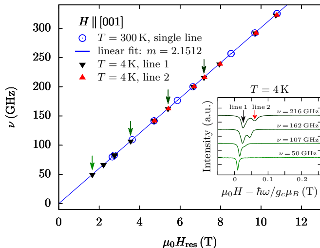
FIG. 6. Frequency-field dependence of resonance positions for CPB at 300 K and 4 K with external magnetic field oriented along the c axis. Arrows in the main plot indicate the resonance positions of the selected ESR spectra shown in the inset, recorded at 4 K and, for a better comparison, shifted horizontally by the paramagnetic resonance frequency as well as vertically by arbitrary amounts.
