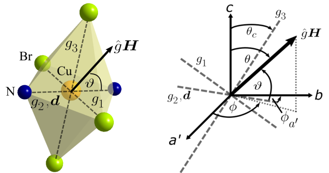
FIG. 2. Left: Local coordinate system of a stretched octahedron formed by four bromine ions (green) and two nitrogen ions (dark blue), surrounding the central copper ion (yellow). Principal axes g_1 , g_2 , and g_3 of the g -tensor \hat{g} coincide with the symmetry axes of the stretched octahedron. The angle between local magnetic field \hat{g}\mathbf{H} and anisotropy axis \mathbf{d} is denoted by \vartheta . Right: Angles of \hat{g}\mathbf{H} ( \theta , \phi ), \mathbf{d} ( 90^\circ , 90^\circ - \phi_{a'} ), and g_3 ( \theta_c , -\phi_{a'} ) with respect to the crystallographic frame ( \mathbf{a}' , \mathbf{b} , \mathbf{c} ). Additionally, the angle \vartheta between \hat{g}\mathbf{H} and \mathbf{d} is shown.
