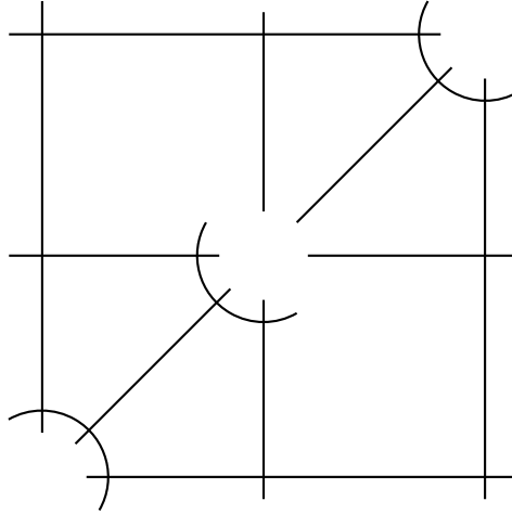
FIGURE 3. The combinatorial structure of \overline{\mathcal{M}}_{0,5} .
