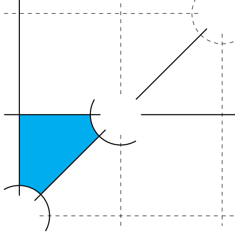
FIGURE 4. The combinatorial structure of \mathcal{M}_{0,5}^\delta .
