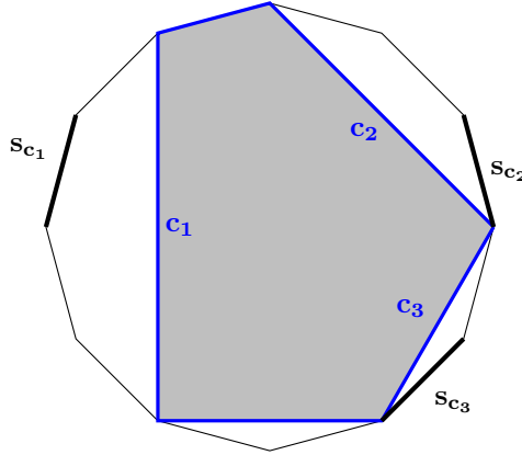
FIGURE 7. An inscribed polygon and a possible choice of matching sides.
