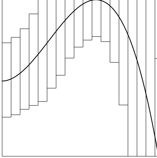
FIGURE 2. Boxes I_i \times J_i .
