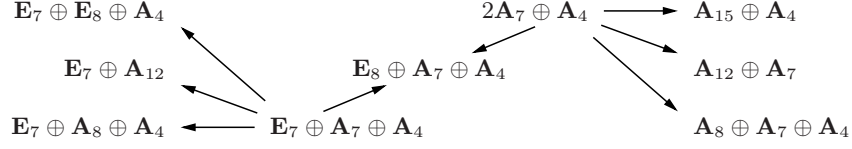
FIGURE 1. The graph \mathfrak{C}_2
