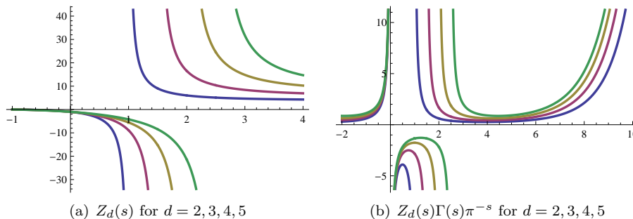
FIGURE 2. The functions Z_d(s) on the real line for various values of d .
