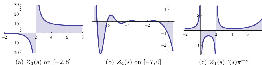
FIGURE 1. Different views on Z_4(s) on the real line.
