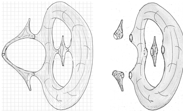
FIGURE 8. (\delta, \eta) -thick components in hyperbolic metric
