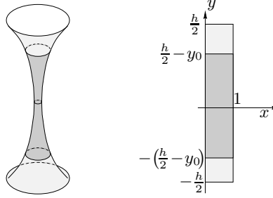
FIGURE 13. Parametrization of a hyperbolic cylinder
