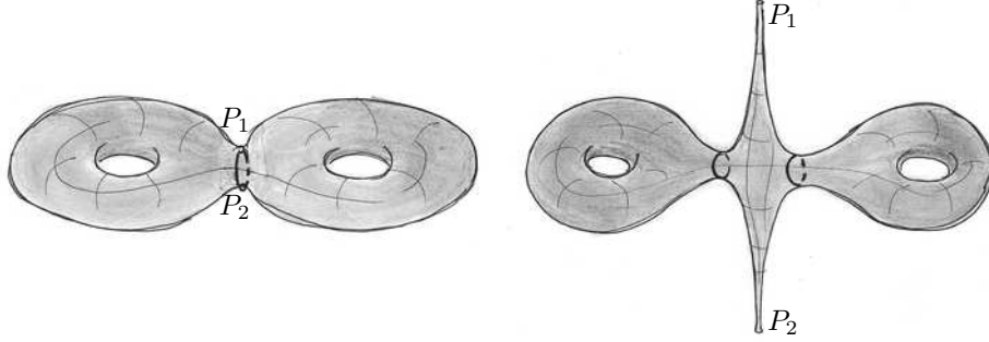
FIGURE 14. A pair of homologous saddle connections in the flat metric produces in the underlying hyperbolic metric a thick component isometric to a sphere with two cusps and with two boundary components represented by short hyperbolic geodesics. The stable curve obtained in the limit has three irreducible components: the two Riemann surfaces underlying S_1 and S_2 and a four-punctured sphere between them.
