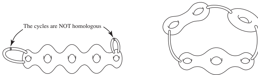
FIGURE 2. Topological pictures for admissible (on the right) and non-admissible (on the left) configurations of cylinders.
