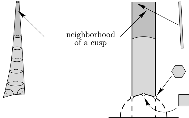
FIGURE 3. Space of flat tori
