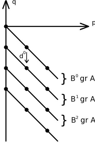
FIGURE 2. The page E^0 of the spectral sequence
