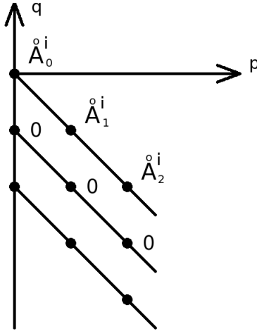
FIGURE 3. The page E^1 of the spectral sequence
