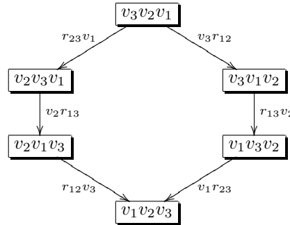
FIGURE 4. Hexagonal diamond
