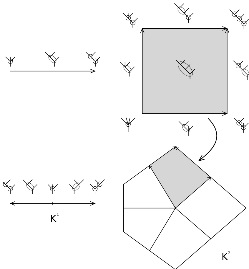
FIGURE 3. K^2 with circled trees
