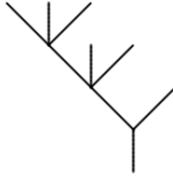
FIGURE 6. Example of a left comb
