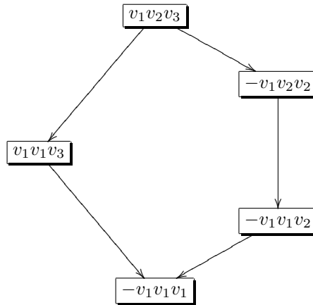
FIGURE 1. Pentagonal diamond
