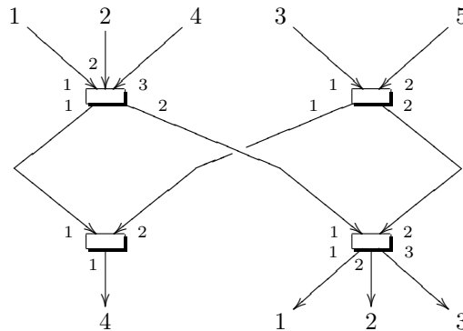
FIGURE 3. Labeled connected graph
