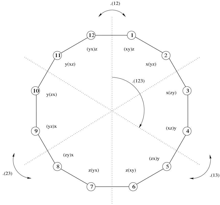
FIGURE 1. The permutoassociahedron
