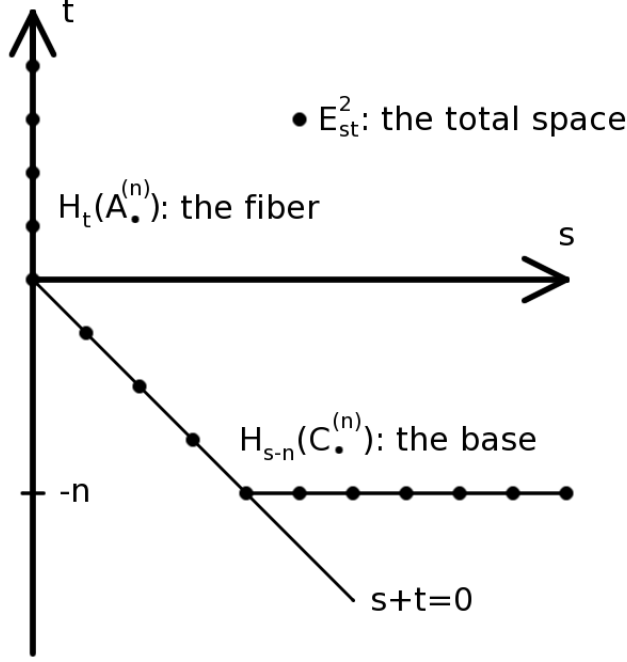
FIGURE 1. The page E_{st}^2 of the spectral sequence
