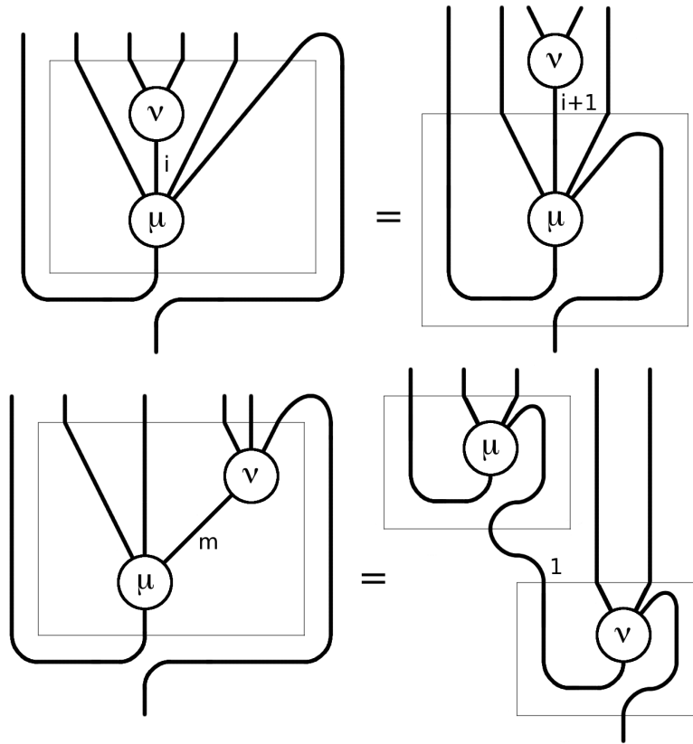
FIGURE 2. \tau(\mu \circ_i \nu) = \tau(\mu) \circ_{i+1} \nu and \tau(\mu \circ_m \nu) = \tau(\nu) \circ_1 \tau(\mu)
