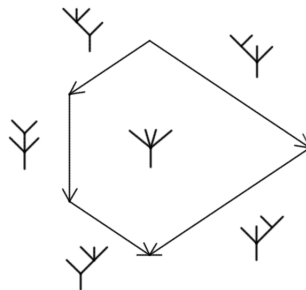
FIGURE 2. Pentagon
