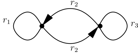
Figure 2: Type [4] \times^2 [4] \mathcal{I} -weighted stable curve
