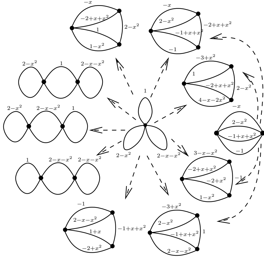
Figure 3: The boundary of the Hilbert modular threefold of discriminant 49.
