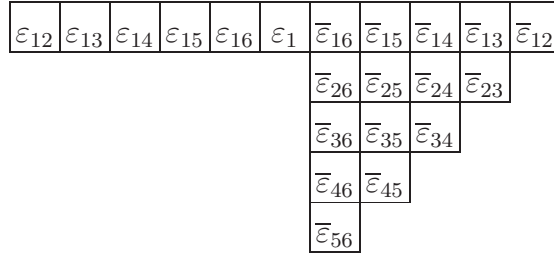
FIGURE 1. The (po)set of commutative roots for \mathfrak{so}_{13}
