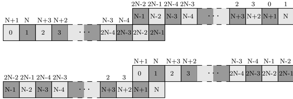
FIGURE 4. Square-tiled M_{2N}(N+2, N-2, N, N) , where N is odd. A square atop a white one is always black and vice versa.
