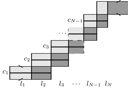
FIGURE 8. A horizontal deformation of the square-tiled cyclic cover M_N(N - 1, 1, N - 1, 1)
