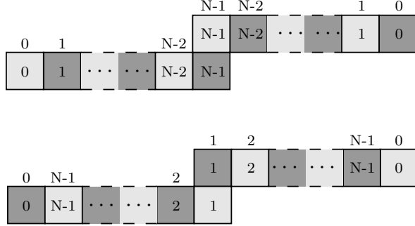
FIGURE 6. Square-tiled M_N(N - 1, 1, N - 1, 1) for even N . A square atop a white one is always black and vice versa.
