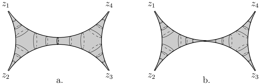
FIGURE 2. Degeneration of \mathbb{CP}^1 with 4 marked points.
