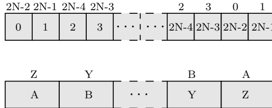
FIGURE 5. Quotient of a square-tiled cyclic cover M_{2N}(N+2, N-2, N, N) over the involution \tau .
