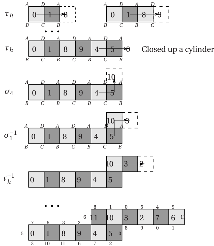
FIGURE 3. Cartoon movie construction of M_6(1, 1, 1, 3) .
