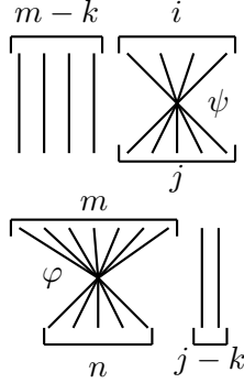
FIGURE 1. Depiction of the partial gluing operation \circ_k where the first k outputs of \psi are composed with the last k inputs of \varphi
