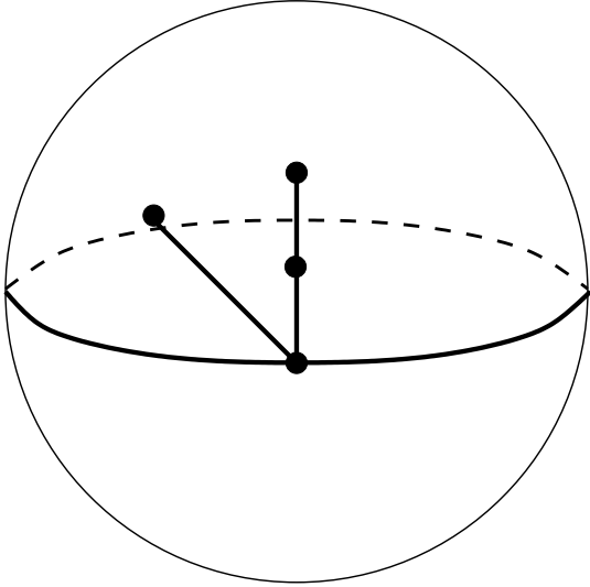
Figure 116: S(4211|71)_+ . Valencies (4, 2, 1, 1|7, 1) . The order of the automorphism group: 1. Dual dessin S(71|4211)_+ , see Figure 47 on the page 31. Belyi function is \beta = \frac{(49z^2 - 90z - 2i\sqrt{7}z + 42 + 2i\sqrt{7})(128z + 5i\sqrt{7} - 119)^2 z^4}{512(16377 + 181i\sqrt{7})(z-1)^7}
