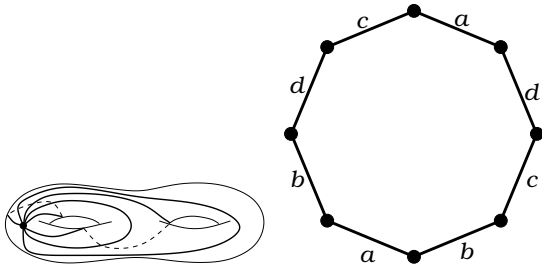
Figure 44: P(8|8)_1A . Valencies (8|8) . The order of the automorphism group: 1. Dual dessin P(8|8)_1A , see Figure 44 on the page 29.
