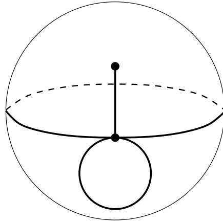
Figure 14: S(51|321) . Valencies (51|3, 2, 1) . The order of the automorphism group: 1. Dual dessin S(321|51) , see Figure 23 on the page 20. Belyi function is \beta = \frac{-64(15z+1)}{3125z^3(z-1)^2(5z-8)} .
