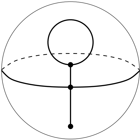
Figure 108: S(431|431)B . Valencies (4, 3, 1|4, 3, 1) . The order of the automorphism group: 1. Dual dessin S(431|431)B , see Figure 108 on the page 51. Belyi function is \beta = \frac{1}{3294172} \frac{(-835+872\sqrt{2})(z-8+5\sqrt{2})(z+8+9\sqrt{2})^3 z^4}{(z+11+8\sqrt{2})(z-1)^3} .
