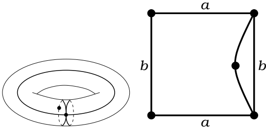
Figure 68: T(62|53) . Valencies (6, 2|5, 3) . The order of the automorphism group: 1. Dual dessin T(53|62) , see Figure 84 on the page 43. Belyi function is \beta = \frac{1}{162}(x^5 + yx^3 + \frac{65}{8}x^4 + 6yx^2 + x^3 - 64x^2 - 16y - 16x + 80) on the curve X : y^2 = \frac{1}{4}(x-1)(4x+5)(x^2 + 4x - 20) . n_0 = \frac{1}{20736} (x+8)^2 x^6 , n_1 = \frac{1}{20736} (x^4 + 8x^3 - 128x - 16)^2
