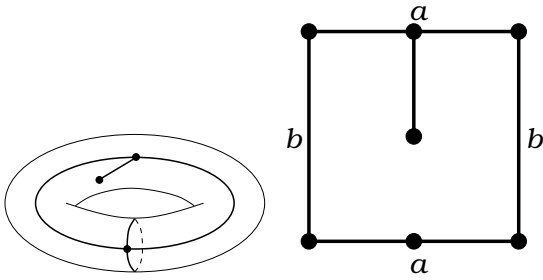
Figure 110: T(431|8)A . Valencies (4, 3, 1|8) . The order of the automorphism group: 1. Dual dessin T(8|431)A , see Figure 37 on the page 27. Belyi function is \beta = -\frac{256}{85766121}(5488x^4 + 14112yx^2 - 26264x^3 + 37548yx - 202741x^2 + 3240y - 73368x - 3240) on the curve X : y^2 = \frac{1}{81}(1 - x)(448x^2 + 1872x + 81) . n_0 = \frac{65536}{62523502209}(4x + 45)(4x + 21)^3x^4 , n_1 = \frac{(4096x^4 + 55296x^3 + 158976x^2 + 55296x - 247617)^2}{62523502209} .
