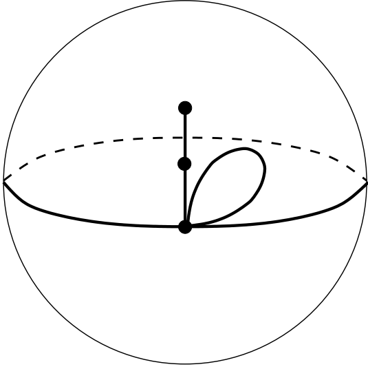
Figure 86: S(521|611) . Valencies (5, 2, 1|6, 1, 1) . The order of the automorphism group: 1. Dual dessin S(611|521) , see Figure 72 on the page 39. Belyi function is \beta = -1/4 \frac{(5z-14)^2(z-4)z^5}{70z^2+24z+9} .
