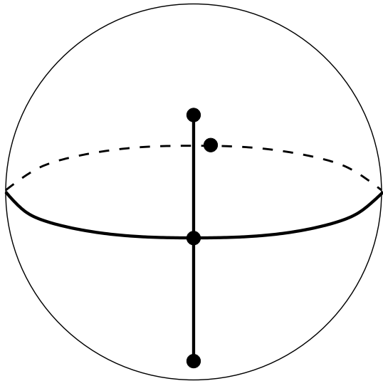
Figure 120: S(4211|44) . Valencies (4, 2, 1, 1|4, 4) . The order of the automorphism group: 2. Dual dessin S(44|4211) , see Figure 97 on the page 48. Belyi function is \beta = 4 \frac{z^2(z^2+2)}{(z^2+1)^4} .
