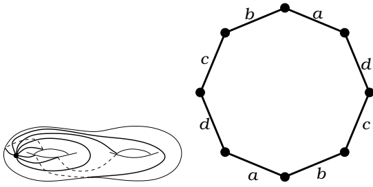
Figure 42: P(8|8)_8 . Valencies (8|8) . The order of the automorphism group: 8. Dual dessin P(8|8)_8 , see Figure 42 on the page 29. Belyi function is (X : y^2 = x^5 - x, \beta = x^4) .
