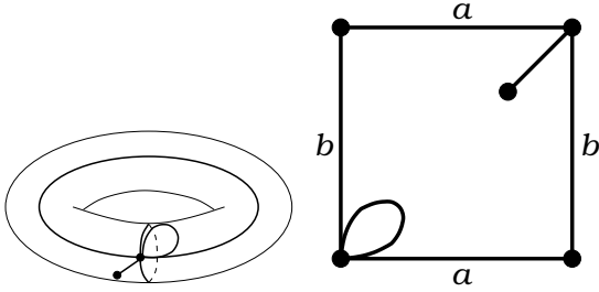
Figure 55: T(71|71)C . Valencies (7, 1, |7, 1) . The order of the automorphism group: 1. Dual dessin T(71|71)C , see Figure 55 on the page 33. Belyi function is \beta = \frac{1}{128} \frac{x^3(7x+y)}{x-1} on the curve X : y^2 = 4x^3 + 13x^2 + 32x . n_0 = -\frac{1}{4096} \frac{x^7(x-8)}{x-1} , n_1 = -\frac{1}{4096} \frac{(x^4-4x^3-8x^2-32x+64)^2}{x-1} .
