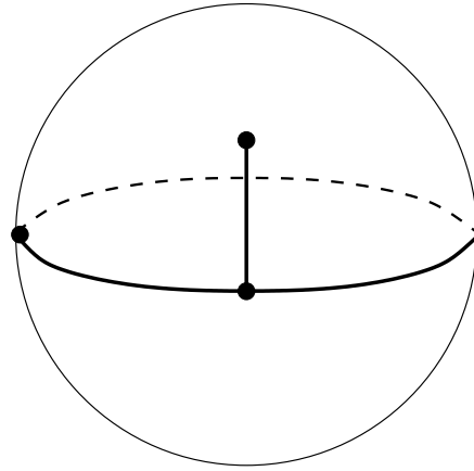
Figure 24: S(321|42) . Valencies (3, 2, 1|4, 2) . The order of the automorphism group: 1. Dual dessin S(42|321) , see Figure 16 on the page 15. Belyi function is \beta = \frac{-4z^3(z-1)^2(z+2)}{(3z-2)^2} .
