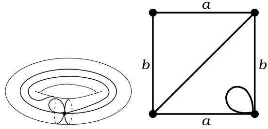
Figure 38: T(8|431)B . Valencies (8|4, 3, 1) . The order of the automorphism group: 1. Dual dessin T(431|8)B , see Figure 111 on the page 52. Belyi function is \beta = -36(81x^4 - 108yx^2 + 288x^3 - 96yx + 308x^2 - 24y + 160x + 32)^{-1} on the curve X : y^2 = \frac{4}{9}(x+1)(9x^2 + 4x + 4) . n_0 = \frac{16}{3} \frac{1}{(x-2)(3x+2)^3x^4} , n_1 = \frac{1}{27} \frac{(27x^4 - 36x^2 - 32x - 20)^2}{(x-2)(3x+2)^3x^4} .
