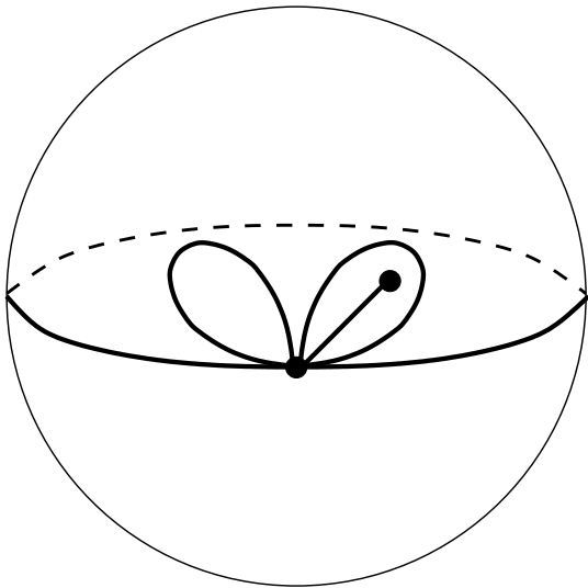
Figure 49: S(71|3311) . Valencies (7, 1|3, 3, 1, 1) . The order of the automorphism group: 1. Dual dessin S(3311|71) , see Figure 126 on the page 59. Belyi function is \beta = -1728 \frac{z}{(1+z^2-5z)^3(49-13z+z^2)} .
