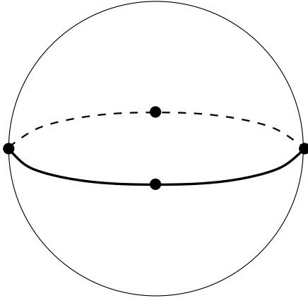
Figure 133: S(2222|44) . Valencies (2, 2, 2, 2|4, 4) . The order of the automorphism group: 8. Dual dessin S(44|2222) , see Figure 99 on the page 48. Belyi function is \beta = \frac{(z^4+1)^2}{4z^4} .
