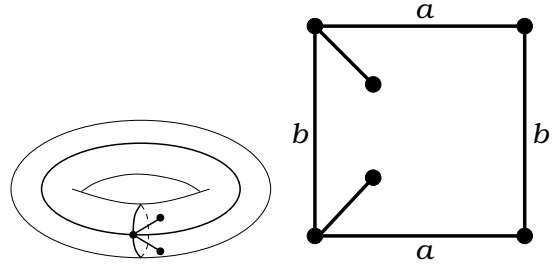
Figure 77: T(611|8)_1A . Valencies (6, 1, 1|8) . The order of the automorphism group: 1. Dual dessin T(8|611)_1A , see Figure 32 on the page 25.
