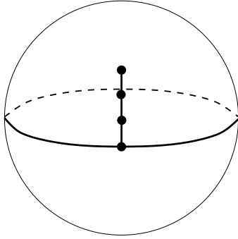
Figure 129: S(3221|71) . Valencies (3, 2, 2, 1|7, 1) . The order of the automorphism group: 1. Dual dessin S(71|3221) , see Figure 50 on the page 31. Belyi function is \beta = 256 \frac{z^3(z+1)(7+28z+24z^2)^2}{48z-1} .
