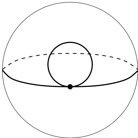
Figure 3: S(4|211) . Valencies (4|2, 1, 1) . The order of the automorphism group: 2. Dual dessin S(211|4) , see Figure 7 on the page 10. Belyi function is \beta = \frac{1}{-4z^2(z^2-1)} .
