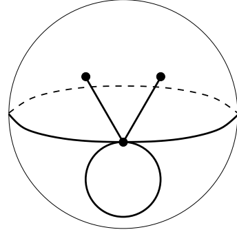
Figure 72: S(611|521) . Valencies (6, 1, 1|5, 2, 1) . The order of the automorphism group: 1. Dual dessin S(521|611) , see Figure 86 on the page 44. Belyi function is \beta = 4 \frac{z^6(9z^2+24z+70)}{(4z-1)(14z-5)^2} .
