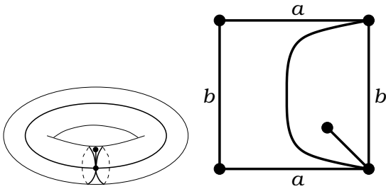
Figure 60: T(71|44) . Valencies (7, 1|4, 4) . The order of the automorphism group: 1. Dual dessin T(44|71) , see Figure 100 on the page 49. Belyi function is \beta = \frac{128}{343}(294x^4 - 28yx^2 + 154x^3 - 7yx + 77x^2 - 2y + 13x + 2) on the curve X : y^2 = 112x^4 + 56x^3 + 37x^2 + 6x + 1 . n_0 = -\frac{65536}{343}(x-2)x^7 , n_1 = -\frac{1}{343}(256x^4 - 256x^3 - 128x^2 - 128x - 13)^2 .
