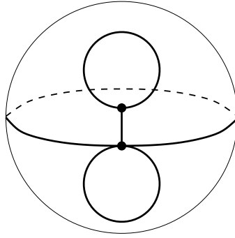
Figure 80: S(53|4211) . Valencies (5, 3|4, 2, 1, 1) . The order of the automorphism group: 1. Dual dessin S(4211|53) , see Figure 119 on the page 55. Belyi function is \beta = \frac{1}{4} \frac{(-1+8z)^3}{(3+z)^2 z^4 (9z^2 + 42z - 5)} .
