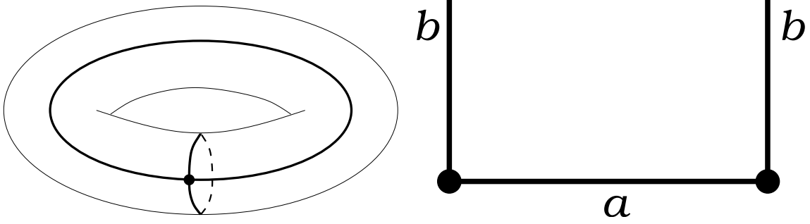
Figure 4: T(4, 4) . Valencies (4|4) . The order of the automorphism group: 4. Dual dessin T(4|4) , see Figure 4 on the page 7. Belyi function is (X : y^2 = x^3 - x, \beta = x^2) .
