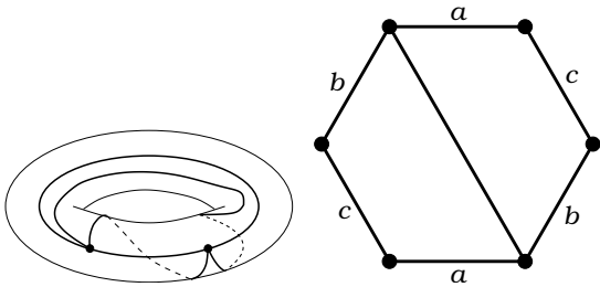
Figure 102: T(44|44)_8 . Valencies (4, 4|4, 4) . The order of the automorphism group: 8. Dual dessin T(44|44)_8 , see Figure 102 on the page 49. Belyi function is (X : y^2 = x^4 - 1, \beta = x^4) .
