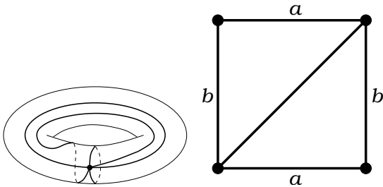
Figure 12: T(6|33) . Valencies (6|3, 3) . The order of the automorphism group: 6. Dual dessin T(33|6) , see Figure 22 on the page 19. Belyi function is (X : y^2 = x^4 - x, \beta = x^3) .
