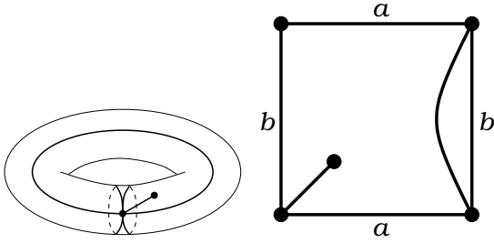
Figure 56: T(71|62)_+ . Valencies (7, 1|6, 2) . The order of the automorphism group: 1. Dual dessin T(62|71)_+ , see Figure 64 on the page 36.
