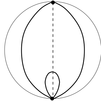
Figure 81: S(53|3221) . Valencies (5, 3|3, 2, 2, 1) . The order of the automorphism group: 1. Dual dessin S(3221|53) , see Figure 131 on the page 60. Belyi function is \beta = 4 \frac{(3z+4)^3 z^5}{(1+7z)(3z+1)^3 (z^2+1)^2} .
