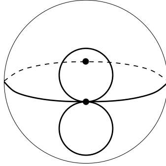
Figure 62: S(62|3311) . Valencies (6, 2|3, 3, 1, 1) . The order of the automorphism group: 2. Dual dessin (3311|62) , see Figure 127 on the page 59. Belyi function is \beta = -64 \frac{z^6}{(-1+3z)(3z+1)(z-1)^3(z+1)^3} .
