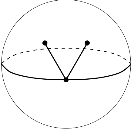
Figure 18: S(411|51) . Valencies (4, 1, 1|5, 1) . The order of the automorphism group: 1. Dual dessin S(51|411) , see Figure 13 on the page 13. Belyi function is \beta = \frac{z^4(z^2+4z+20)}{256(z-1)}
