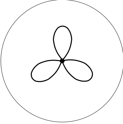
Figure 8: S(6|3111) . Valencies (6|3, 1, 1, 1) . The order of the automorphism group: 3. Dual dessin S(3111|6) , see Figure 25 on the page 21. Belyi function is \beta = \frac{1}{-4z^3(z^3-1)} .
