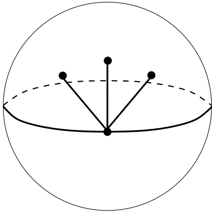
Figure 95: S(5111|71) . Valencies (5, 1, 1, 1|7, 1) . The order of the automorphism group: 1. Dual dessin S(71|5111) , see Figure 46 on the page 30. Belyi function is \beta = \frac{1}{16384} \frac{z^5(1225z^3 - 3216z^2 + 2912z - 896)}{(z-1)^7} .
