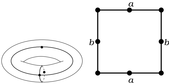
Figure 114: T(422|8)_4 . Valencies (4, 2, 2|8) . The order of the automorphism group: 4. Dual dessin T(8|422)_4 , see Figure 39 on the page 28. Belyi function is (X : y^2 = x(x-1)(x+1), \beta = -4x^2(x-1)(x+1)) .
