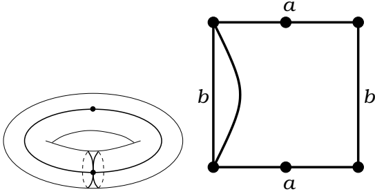
Figure 66: T(62|62)_2 . Valencies (6, 2|6, 2) . The order of the automorphism group: 2. Dual dessin T(62|62)_2 , see Figure 66 on the page 38. Belyi function is (X : y^2 = x(x+8)(x-1)) , \beta = \frac{1}{64} \frac{x^3(x+8)}{x-1} .
