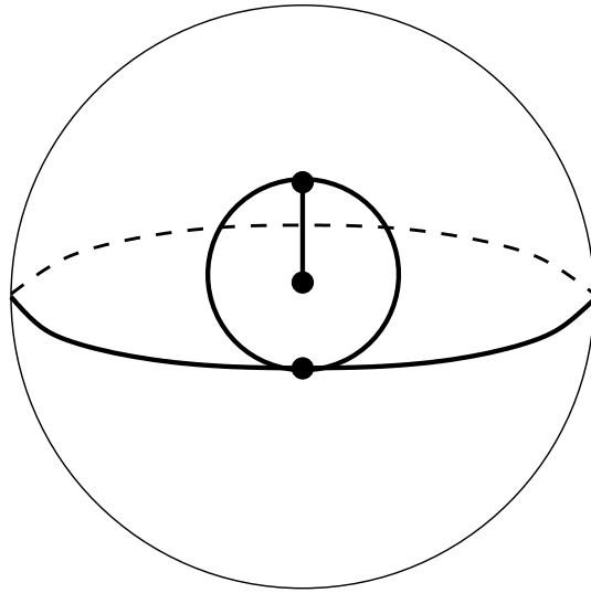
Figure 107: S(431|431)A . Valencies (4, 3, 1|4, 3, 1) . The order of the automorphism group: 1. Dual dessin S(431|431)A , see Figure 107 on the page 51. Belyi function is \beta = \frac{1}{3294172} \frac{(835+872\sqrt{2})(-z+8+5\sqrt{2})(-z-8+9\sqrt{2})^3 z^4}{(-z-11+8\sqrt{2})(z-1)^3} .
