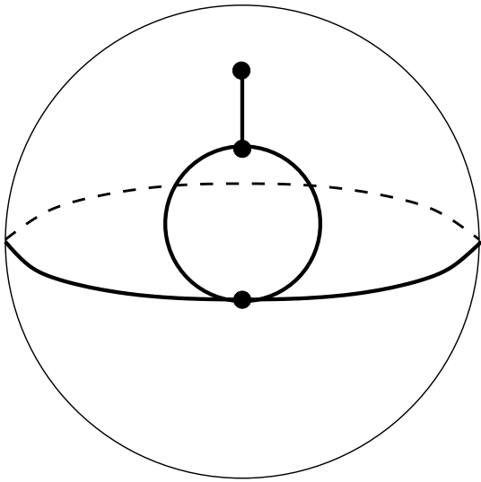
Figure 106: S(431|521) . Valencies (4, 3, 1|5, 2, 1) . The order of the automorphism group: 1. Dual dessin S(521|431) , see Figure 90 on the page 45. Belyi function is \beta = -1/16 \frac{(4z-7)^3(4z-15)z^4}{(3z+1)(7z-6)^2} .
