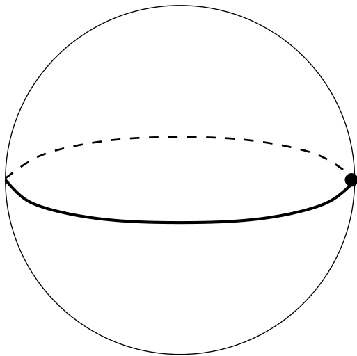
Figure 1: S(2|11) . Valencies (2|1,1) . The order of the automorphism group: 2. Dual dessin S(11|2) , see Figure 2 on the page 5. Belyi function is \beta = \frac{z^2}{z^2-1} .
