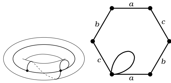
Figure 83: T(53|71)B . Valencies (5, 3|7, 1) . The order of the automorphism group: 1. Dual dessin T(71|53)B , see Figure 59 on the page 34.
