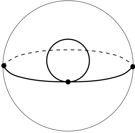
Figure 112: S(422|431) . Valencies (4, 2, 2|4, 3, 1) . The order of the automorphism group: 1. Dual dessin S(431|422) , see Figure 109 on the page 51. Belyi function is \beta = -1/4 \frac{(z^2+4z+6)^2 z^4}{(z+1)^4(4z+1)} .
