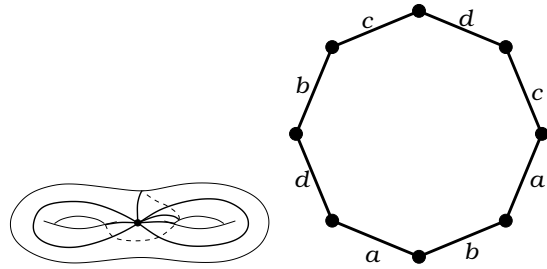
Figure 45: P(8|8)_1B . Valencies (8|8) . The order of the automorphism group: 1. Dual dessin P(8|8)_1B , see Figure 45 on the page 29.
