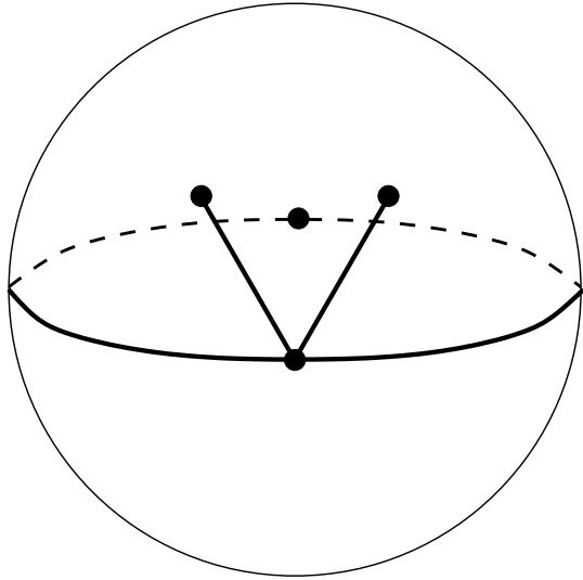
Figure 118: S(4211|62) . Valencies (4, 2, 1, 1|6, 2) . The order of the automorphism group: 1. Dual dessin S(62|4211) , see Figure 61 on the page 36. Belyi function is \beta = -108 \frac{z^4(1+2z+3z^2)(-1+3z)^2}{(-1+4z)^2} .
