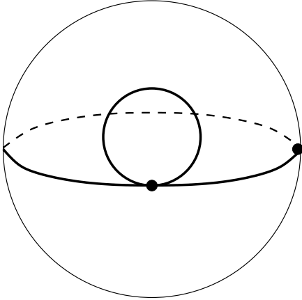
Figure 16: S(42|321) . Valencies (4, 2|3, 2, 1) . The order of the automorphism group: 1. Dual dessin S(321|42) , see Figure 24 on the page 20. Belyi function is \beta = \frac{-(3z-2)^2}{4z^3(z-1)^2(z+2)} .
