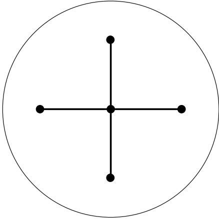
Figure 121: S(4|1111|8) . Valencies (4, 1, 1, 1, 1|8) . The order of the automorphism group: 4. Dual dessin S(8|41111) , see Figure 28 on the page 24. Belyi function is \beta = -4z^4(z - 1)(z + 1)(z^2 + 1) .
