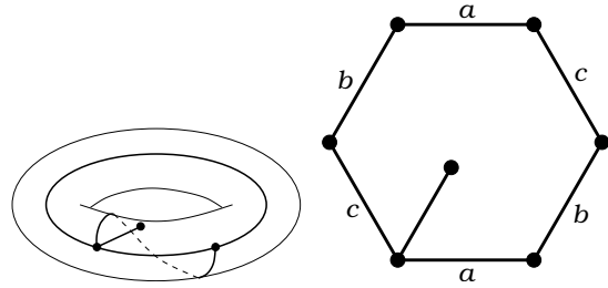
Figure 111: T(431|8)B . Valencies (4, 3, 1|8) . The order of the automorphism group: 1. Dual dessin T(8|431)B , see Figure 38 on the page 27. Belyi function is \beta = -9/4x^4 + 3yx^2 - 8x^3 + 8/3yx - \frac{77}{9}x^2 + 2/3y - \frac{40}{9}x - \frac{8}{9} on the curve X : y^2 = \frac{4}{9}(x + 1)(9x^2 + 4x + 4) . n_0 = \frac{3}{16}(x - 2)(3x + 2)^3x^4 , n_1 = \frac{1}{144}(27x^4 - 36x^2 - 32x - 20)^2 .
