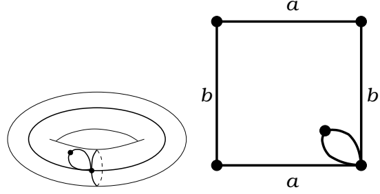
Figure 67: T(62|62)_1 . Valencies (6, 2|6, 2) . The order of the automorphism group: 1. Dual dessin T(62|62)_1 , see Figure 67 on the page 38. Belyi function is \beta = -\frac{1}{432} \frac{(18x^3 - 810x^2 + 9342x - 5382)y}{(4x-89)^2} - \frac{1}{432} \frac{4x^5 - 103x^4 - 1172x^3 + 28030x^2 + 126536x - 295247}{(4x-89)^2} on the curve X : y^2 = 4(x-2)(x^2 + 2x + 73) . n_0 = \frac{1}{186624} \frac{(x-29)^2(x-5)^6}{(4x-89)^2} , n_1 = \frac{1}{186624} \frac{(x^4 - 44x^3 + 510x^2 - 572x + 35161)^2}{(4x-89)^2} .
