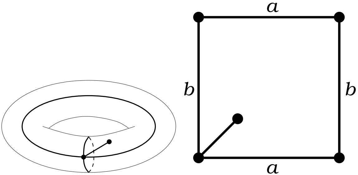
Figure 15: T(51|6) . Valencies (5, 1|6) . The order of the automorphism group: 1. Dual dessin T(6|51) , see Figure 10 on the page 12. Belyi function is \beta = \frac{25x^3 - 270yx - 255x^2 + 216y + 522x - 216}{1250} on the curve X : y^2 = -\frac{5}{18}x^3 + \frac{29}{36}x^2 - \frac{7}{3}x + 1 . n_0 = \frac{x^5(12+x)}{2500} , n_1 = \frac{(x^3+6x^2-18x+58)^2}{2500} .
