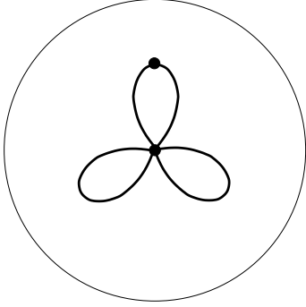
Figure 61: S(62|4211) . Valencies (6, 2|4, 2, 1, 1) . The order of the automorphism group: 1. Dual dessin S(4211|62) , see Figure 118 on the page 55. Belyi function is \beta = -\frac{1}{108} \frac{z^6(z-4)^2}{(z^2+2z+3)(z-3)^2}
