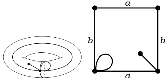
Figure 52: T(71|71)A_- . Valencies (7, 1|7, 1) . The order of the automorphism group: 1. Dual dessin T(71|71)A_+ , see Figure 51 on the page 32.
