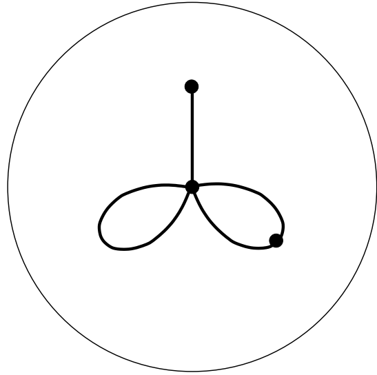
Figure 89: S(521|521)B_- . Valencies (5, 2, 1|5, 2, 1) . The order of the automorphism group: 1. Dual dessin S(521|521)B_- , see Figure 89 on the page 45. Belyi function is \beta = \{16 \frac{(391+550\nu+455\nu^2)(z+2\nu)(z+1)^2z^5}{(16z-\nu+7\nu^2-4)(-8z+3\nu+3\nu^2-4)^2}, 7\nu^3 + 2\nu^2 - \nu - 4 = 0, \text{Im}\nu > 0\} .
