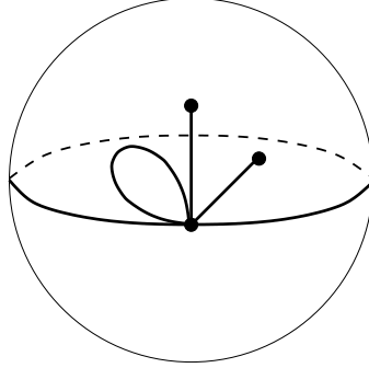
Figure 71: S(611|611)_1 . Valencies (6, 1, 1|6, 1, 1) . The order of the automorphism group: 1. Dual dessin S(611|611)_1 , see Figure 71 on the page 39. Belyi function is \beta = -\frac{27}{4} \frac{(3z^2+6z+7)z^6}{21z^2-12z+4} .
