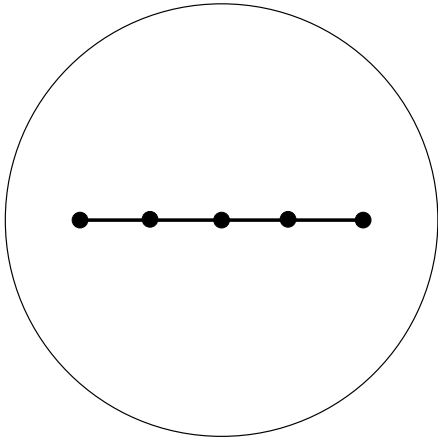
Figure 134: S(22211|8) . Valencies (2, 2, 2, 1, 1|8) . The order of the automorphism group: 2. Dual dessin S(8|22211) , see Figure 30 on the page 24. Belyi function is \beta = -4z^2(z^2 - 2)(z - 1)^2(z + 1)^2
