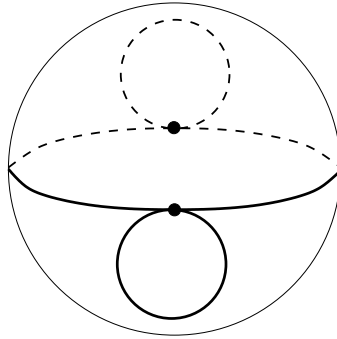
Figure 98: S(44|3311) . Valencies (4, 4|3, 3, 1, 1) . The order of the automorphism group: 2. Dual dessin S(3311|44) , see Figure 128 on the page 59. Belyi function is \beta = -432 \frac{z^4}{(2z^2+10z-1)(2z^2+2z-1)^3} .
