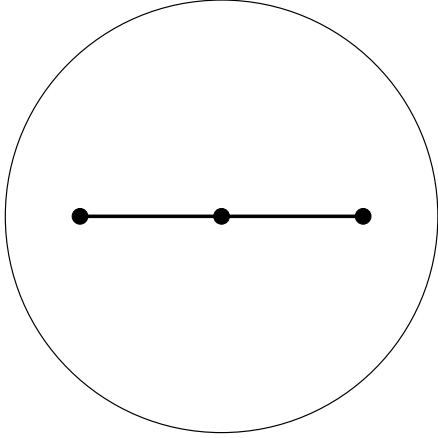
Figure 7: S(211|4) . Valencies (2, 1, 1|4) . The order of the automorphism group: 2. Dual dessin S(4|211) , see Figure 3 on the page 6. Belyi function is \beta = -4z^2(z^2 - 1) .
