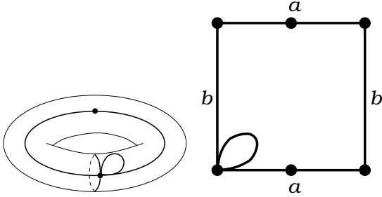
Figure 64: T(62|71)_+ . Valencies (6, 2|7, 1) . The order of the automorphism group: 1. Dual dessin T(71|62)_+ , see Figure 56 on the page 34.
