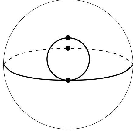
Figure 113: S(422|422) . Valencies (4, 2, 2|4, 2, 2) . The order of the automorphism group: 2. Dual dessin S(422|422) , see Figure 113 on the page 53. Belyi function is \beta = -1/4 \frac{(z^2-2)^2 z^4}{(z-1)^2(z+1)^2} .
