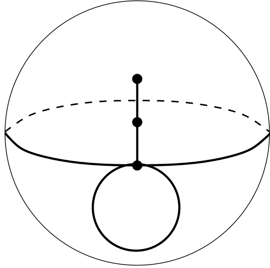
Figure 87: S(521|521)A . Valencies (5, 2, 1|5, 2, 1) . The order of the automorphism group: 1. Dual dessin S(521|521)A , see Figure 87 on the page 44. Belyi function is \beta = \{16 \frac{(391+550\nu+455\nu^2)(z+2\nu)(z+1)^2z^5}{(16z-\nu+7\nu^2-4)(-8z+3\nu+3\nu^2-4)^2}, 7\nu^3 + 2\nu^2 - \nu - 4 = 0, \nu > 0\} .
