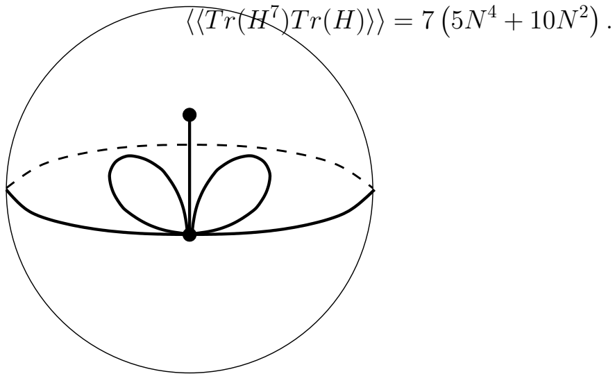
Figure 46: S(71|5111) . Valencies (7, 1|5, 1, 1, 1) . The order of the automorphism group: 1. Dual dessin S(5111|71) , see Figure 95 on the page 47. Belyi function is \beta = \frac{16384z(z-1)^7}{896z^3 - 2912z^2 + 3216z - 1225} .
