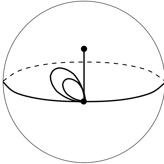
Figure 48: S(71|4211)_- . Valencies (7, 1|4, 2, 1, 1) . The order of the automorphism group: 1. Dual dessin S(4211|71)_- , see Figure 117 on the page 54. Belyi function is \beta = \frac{-7340032(-i\sqrt{7}+21)z(z-1)^7}{(896z^2-1904z-48iz\sqrt{7}+1029+49i\sqrt{7})(112z-119+5i\sqrt{7})^2}
