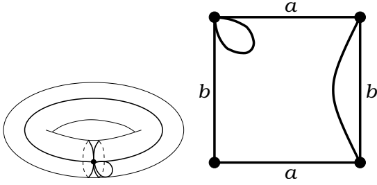
Figure 35: T(8|521)A_- . Valencies (8|5, 2, 1) . The order of the automorphism group: 1. Dual dessin T(521|8)A_- , see Figure 93 on the page 46.
