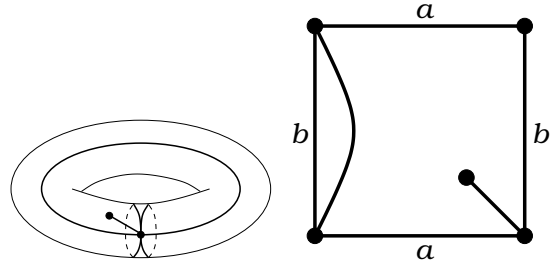
Figure 57: T(71|62)_- . Valencies (7, 1|6, 2) . The order of the automorphism group: 1. Dual dessin T(62|71)_- , see Figure 65 on the page 36.
