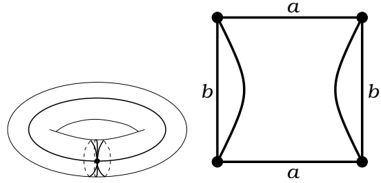
Figure 40: T(8|422)_2 . Valencies (8|4, 2, 2) . The order of the automorphism group: 2. Dual dessin T(422|8)_2 , see Figure 115 on the page 53. Belyi function is X : y^2 = 4x^3 - 4x^2 - x, \beta = \frac{1}{16x^2(x-1)^2} .
