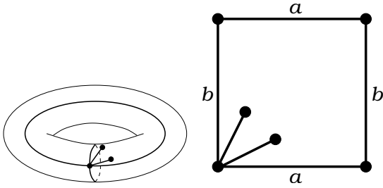
Figure 78: T(611|8)_1B . Valencies (6, 1, 1|8) . The order of the automorphism group: 1. Dual dessin T(8|611)_1B , see Figure 33 on the page 25.
