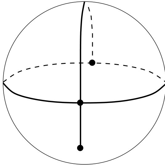
Figure 109: S(431|422) . Valencies (4, 3, 1|4, 2, 2) . The order of the automorphism group: 1. Dual dessin S(422|431) , see Figure 112 on the page 53. Belyi function is \beta = -4 \frac{(z+1)^4 z^3 (z+4)}{(6z^2+4z+1)^2} .
