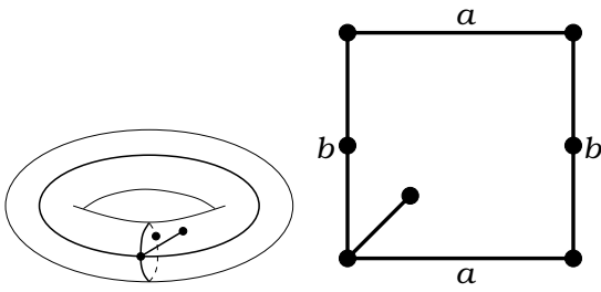
Figure 92: T(521|8)A_+ . Valencies (5, 2, 1|8) . The order of the automorphism group: 1. Dual dessin T(8|521)A_+ , see Figure 34 on the page 26.
