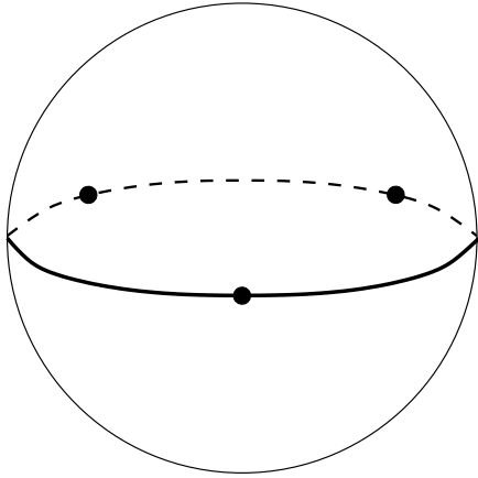
Figure 26: S(222|33) . Valencies (2, 2, 2|3, 3) . The order of the automorphism group: 6. Dual dessin S(33|222) , see Figure 21 on the page 18. Belyi function is \beta = \frac{-(z^3-1)^2}{4z^3} .
