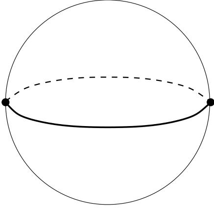
Figure 6: S(22|22) . Valencies (2, 2|2, 2) . The order of the automorphism group: 4. Dual dessin S(22|22) , see Figure 6 on the page 9. Belyi function is \beta = \frac{(z^2-1)^2}{-4z^2} .
