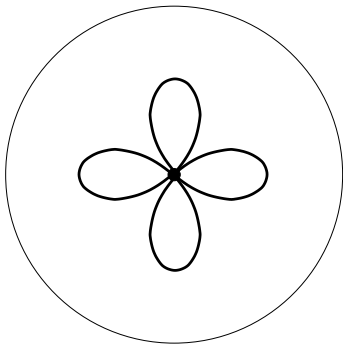
Figure 28: S(8|41111) . Valencies (8|4, 1, 1, 1, 1) . The order of the automorphism group: 4. Dual dessin S(41111|8) , see Figure 121 on the page 56. Belyi function is \beta = \frac{z^8}{4(z-1)(z+1)(z^2+1)}
