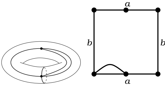
Figure 84: T(53|62) . Valencies (5, 3|6, 2) . The order of the automorphism group: 1. Dual dessin T(62|53) , see Figure 68 on the page 38. Belyi function is \beta = 1296(8yx^3 + 48yx^2 - 128y + 8x^5 + 65x^4 + 8x^3 - 512x^2 - 128x + 640)^{-1} on the curve X : y^2 = \frac{1}{4}(x-1)(4x+5)(x^2+4x-20) . n_0 = 20736 \frac{1}{(x+8)^2x^6} , n_1 = \frac{(x^4+8x^3-128x-16)^2}{(x+8)^2x^6} .
