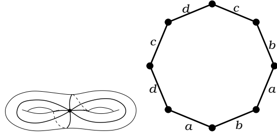
Figure 43: P(8|8)_2 . Valencies (8|8) . The order of the automorphism group: 2. Dual dessin P(8|8)_2 , see Figure 43 on the page 29. Belyi function is \beta = -(-xy + x^4 - 2x^2 + 1)^2 on the curve X : y^2 = (x^2 - 2)(x^4 - 2x^2 + 2) . n_0 = 1 , n_1 = 4(x - 1)^4(x + 1)^4 .
