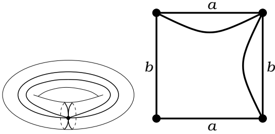
Figure 39: T(8|422)_4 . Valencies (8|4, 2, 2) . The order of the automorphism group: 4. Dual dessin T(422|8)_4 , see Figure 114 on the page 53. Belyi function is (X : y^2 = x^3 - x, \beta = \frac{1}{4} \frac{x^4}{(x-1)(x+1)}) .
