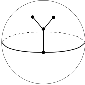
Figure 126: S(3311|71) . Valencies (3, 3, 1, 1|7, 1) . The order of the automorphism group: 1. Dual dessin S(71|3311) , see Figure 49 on the page 31. Belyi function is \beta = \frac{-1}{1728} \frac{(1+z^2-5z)^3(49z^2-13z+1)}{z^7}
