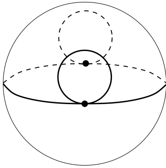
Figure 97: S(44|4211) . Valencies (4, 4|4, 2, 1, 1) . The order of the automorphism group: 2. Dual dessin S(4211|44) , see Figure 120 on the page 55. Belyi function is \beta = 1/4 \frac{(z^2+1)^4}{z^4(2z^2+1)} .
