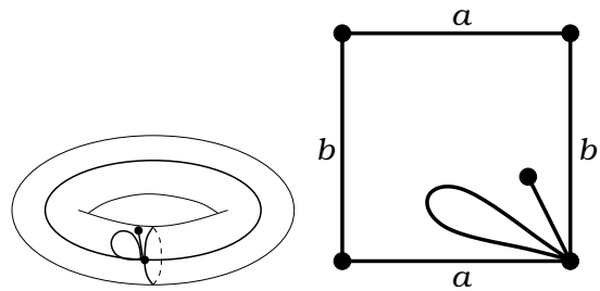
Figure 54: T(71|71)B_- . Valencies (7, 1|7, 1) . The order of the automorphism group: 1. Dual dessin T(71|71)B_- , see Figure 54 on the page 32. Belyi function can be seen below.
