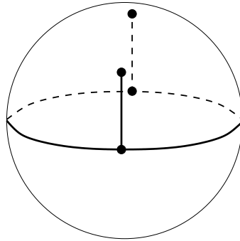
Figure 127: S(3311|62) . Valencies (3, 3, 1, 1|6, 2) . The order of the automorphism group: 2. Dual dessin S(62|3311) , see Figure 62 on the page 36. Belyi function is \beta = \frac{-1}{64} \frac{(z-3)(3+z)(z-1)^3(z+1)^3}{z^2}
