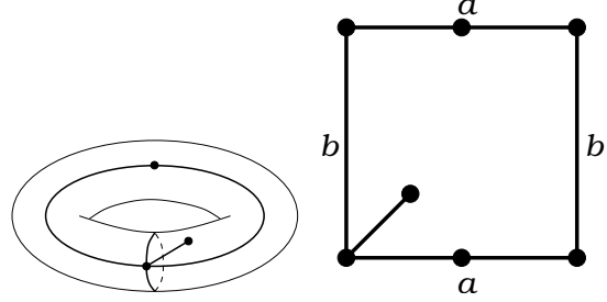
Figure 93: T(521|8)A_- . Valencies (5, 2, 1|8) . The order of the automorphism group: 1. Dual dessin T(8|521)A_- , see Figure 35 on the page 26.
