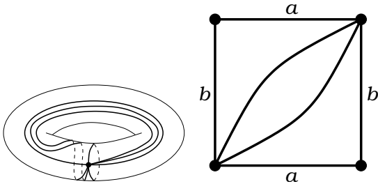
Figure 41: T(8|332) . Valencies (8|3, 3, 2) . The order of the automorphism group: 2. Dual dessin T(332|8) , see Figure 125 on the page 58. Belyi function is X : y^2 = x(x-1)(3x^2 + 8x + 16), \beta = \frac{27}{256} \frac{x^4}{x-1} .
