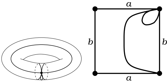
Figure 37: T(8|431)A . Valencies (8|4, 3, 1) . The order of the automorphism group: 1. Dual dessin T(431|8)A , see Figure 110 on the page 52. Belyi function is \beta = -\frac{85766121}{256}(5488x^4 + 14112yx^2 - 26264x^3 + 37548yx - 202741x^2 + 3240y - 73368x - 3240)^{-1} on the curve X : y^2 = \frac{1}{81}(1-x)(448x^2 + 1872x + 81) . n_0 = \frac{62523502209}{65536} \frac{1}{x^4(4x+45)(4x+21)^3} , n_1 = \frac{(4096x^4 + 55296x^3 + 158976x^2 + 55296x - 247617)^2}{65536x^4(4x+45)(4x+21)^3} .
