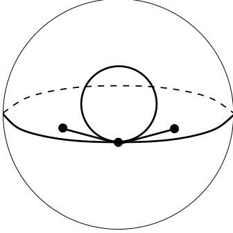
Figure 70: S(611|611)_2 . Valencies (6, 1, 1|6, 1, 1) . The order of the automorphism group: 2. Dual dessin S(611|611)_2 , see Figure 70 on the page 39. Belyi function is \beta = -4 \frac{(z^2-2)z^6}{4z^2+1} .
