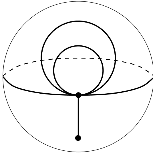
Figure 50: S(71|3221) . Valencies (7, 1|3, 2, 2, 1) . The order of the automorphism group: 1. Dual dessin S(3221|71) , see Figure 129 on the page 60. Belyi function is \beta = -\frac{1}{256} \frac{z^7(-48+z)}{(z+1)(7z^2+28z+24)^2}
