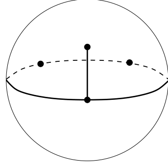
Figure 131: S(3221|53) . Valencies (3, 2, 2, 1|5, 3) . The order of the automorphism group: 1. Dual dessin S(53|3221) , see Figure 81 on the page 42. Belyi function is \beta = \frac{1}{4} \frac{(z+7)(3+z)^3(z^2+1)^2}{(3+4z)^3} .
