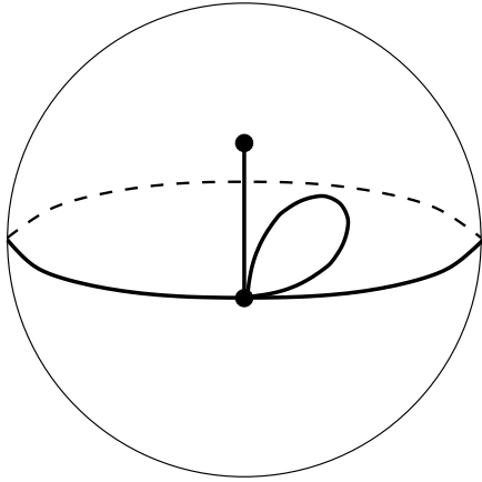
Figure 13: S(51|411) . Valencies (5, 1|4, 1, 1) . The order of the automorphism group: 1. Dual dessin S(411|51) , see Figure 18 on the page 17. Belyi function is \beta = \frac{256(z-1)}{z^4(z^2+4z+20)} .
