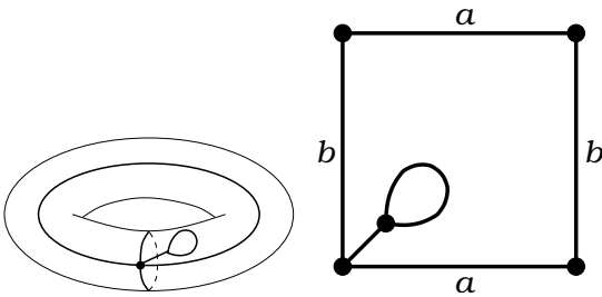
Figure 82: T(53|71)A . Valencies (5, 3|7, 1) . The order of the automorphism group: 1. Dual dessin T(71|53)A , see Figure 58 on the page 34.
