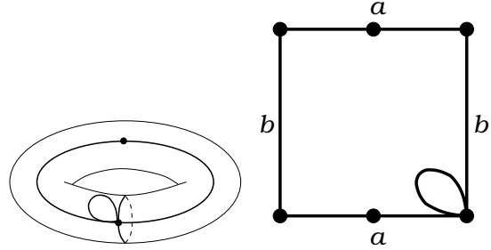
Figure 65: T(62|71)_- . Valencies (6, 2|7, 1) . The order of the automorphism group: 1. Dual dessin T(71|62)_- , see Figure 57 on the page 34.
