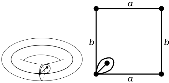
Figure 58: T(71|53)A . Valencies (7, 1|5, 3) . The order of the automorphism group: 1. Dual dessin T(53|71)A , see Figure 82 on the page 42.
