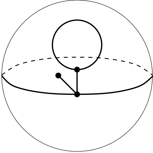
Figure 104: S(431|611)_+ . Valencies (4, 3, 1|6, 1, 1) . The order of the automorphism group: 1. Dual dessin S(611|431)_+ , see Figure 73 on the page 40. Belyi function is \beta = -\frac{49}{4} \frac{(87i\sqrt{3}+211)(z-1)^3(-7z-3+2i\sqrt{3})z^4}{686z^2-672z+56i\sqrt{3}z-57i\sqrt{3}-51} .
