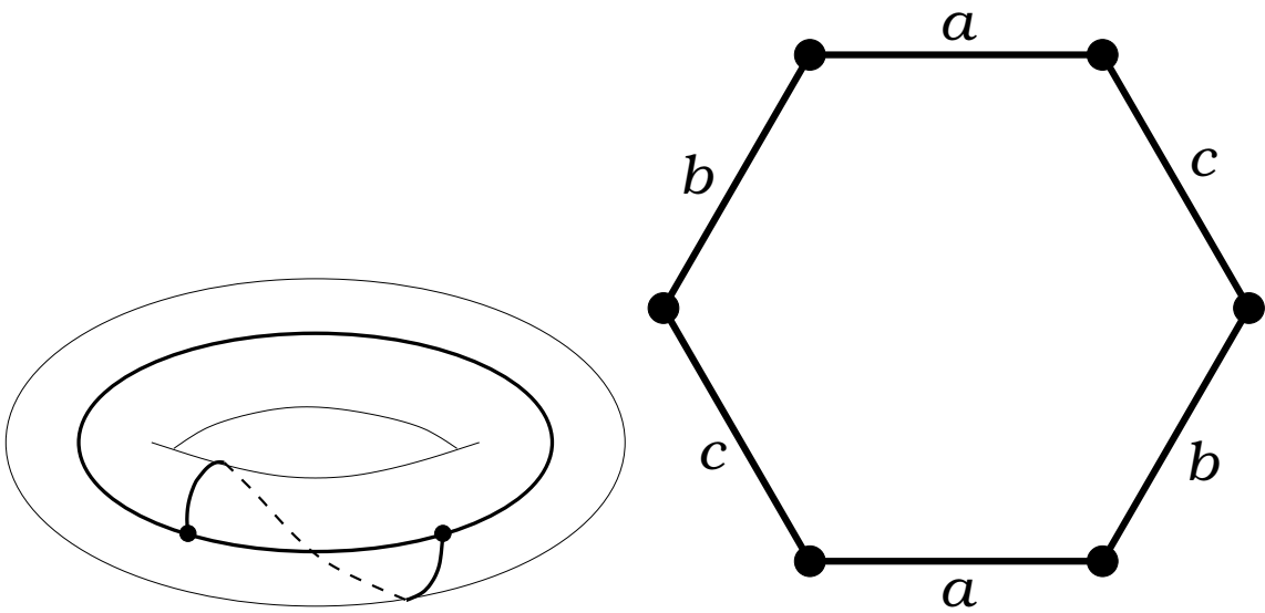
Figure 22: T(33|6) . Valencies (3, 3|6) . The order of the automorphism group: 6. Dual dessin T(6|33) , see Figure 12 on the page 12. Belyi function is (X : y^2 = x^3 - 1, \beta = x^3) .
