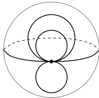
Figure 30: S(8|22211) . Valencies (8|2, 2, 2, 1, 1) . The order of the automorphism group: 2. Dual dessin S(22211|8) , see Figure 134 on the page 63. Belyi function is \beta = \frac{1}{-4z^2(z^2-2)(z-1)^2(z+1)^2}
