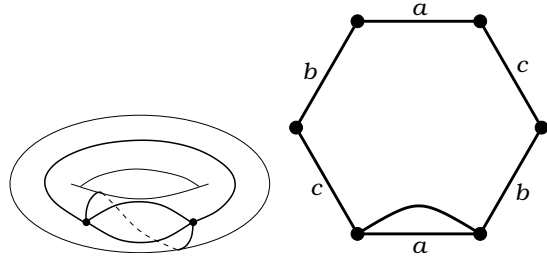
Figure 101: T(44|62) . Valencies (4, 4|6, 2) . The order of the automorphism group: 2. Dual dessin T(62|44) , see Figure 69 on the page 38. Belyi function is (X : y^2 = (x - 1)(3x^2 + 8x + 16), \beta = \frac{27}{256} \frac{x^4}{x-1}) .
