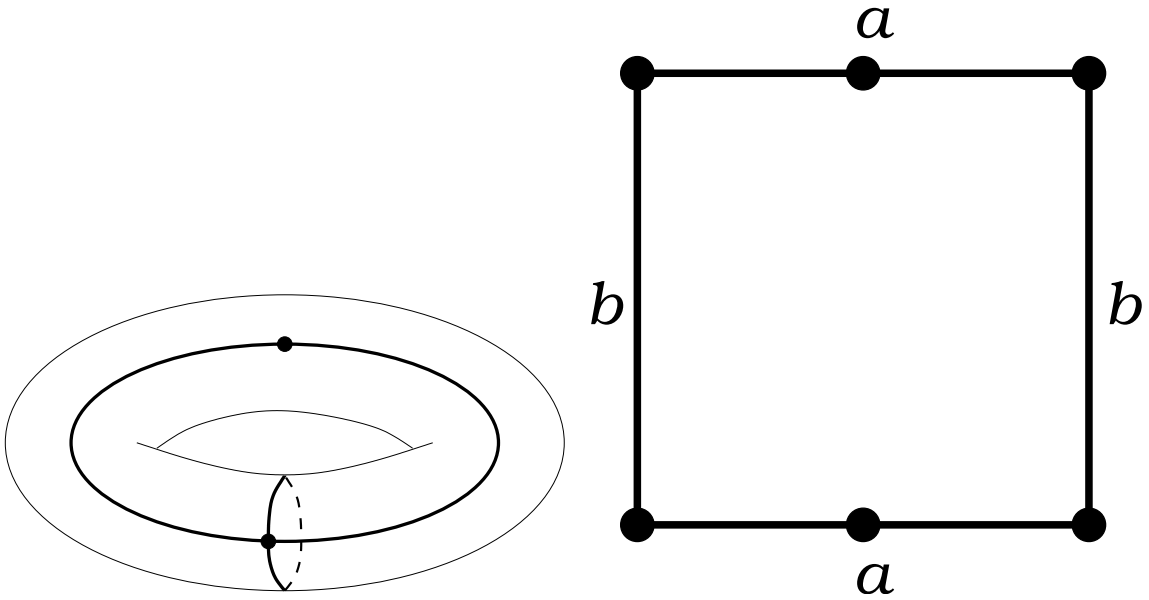
Figure 17: T(42|6) . Valencies (4, 2|6) . The order of the automorphism group: 2. Dual dessin T(6|42) , see Figure 11 on the page 12. Belyi function is (X : y^2 = 4x^3 - 39x + 35, \beta = \frac{(x-1)^2(2x+7)}{27}) .
