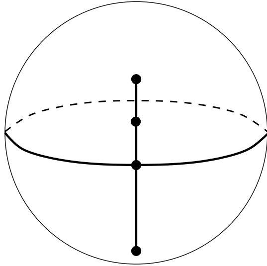
Figure 119: S(4211|53) . Valencies (4, 2, 1, 1|5, 3) . The order of the automorphism group: 1. Dual dessin S(53|4211) , see Figure 80 on the page 42. Belyi function is \beta = 4 \frac{(3z+1)^2(-9-42z+5z^2)}{(z-8)^3z^5} .
