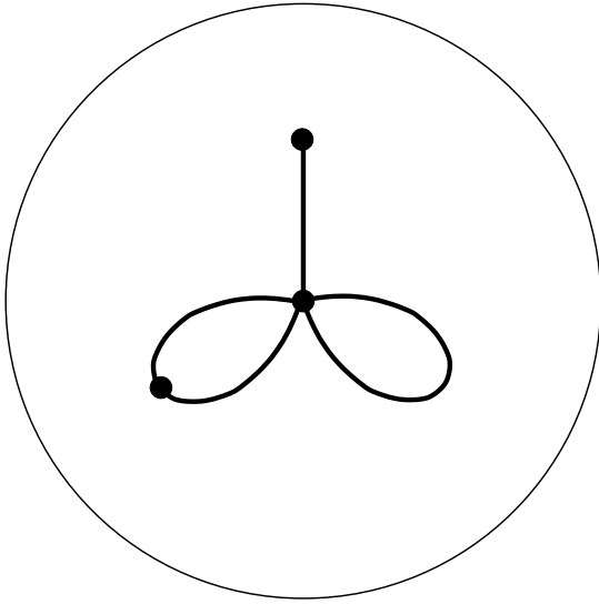
Figure 88: S(521|521)B_+ . Valencies (5, 2, 1|5, 2, 1) . The order of the automorphism group: 1. Dual dessin S(521|521)B_+ , see Figure 88 on the page 45. Belyi function is \beta = \{16 \frac{(391+550\nu+455\nu^2)(z+2\nu)(z+1)^2z^5}{(16z-\nu+7\nu^2-4)(-8z+3\nu+3\nu^2-4)^2}, 7\nu^3 + 2\nu^2 - \nu - 4 = 0, \text{Im}\nu < 0\} .
