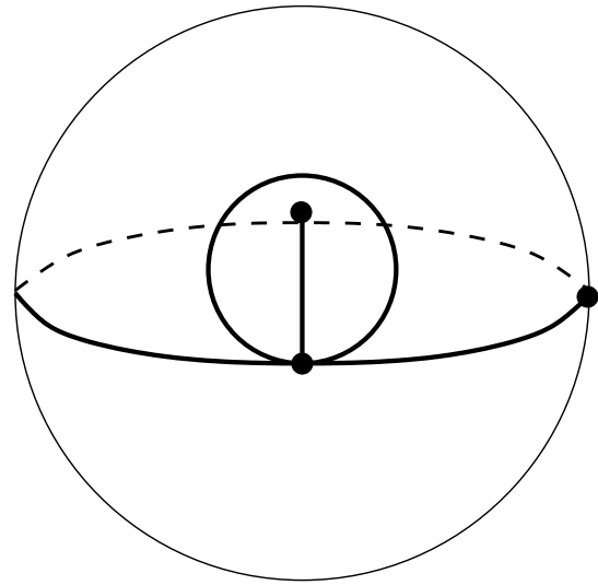
Figure 91: S(521|332) . Valencies (5, 2, 1|3, 3, 2) . The order of the automorphism group: 1. Dual dessin S(332|521) , see Figure 123 on the page 57. Belyi function is \beta = \frac{27}{4} \frac{z^5(7z+2)^2(11z-4)}{(6z^2-1)^3(4z+1)^2} .
