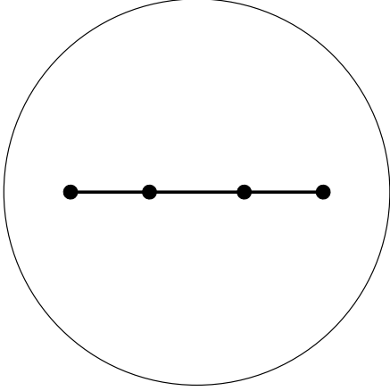
Figure 27: S(2211|6) . Valencies (2, 2, 1, 1|6) . The order of the automorphism group: 2. Dual dessin S(6|2211) , see Figure 9 on the page 11. Belyi function is \beta = -(4z^2 - 1)^2(z^2 - 1) .
