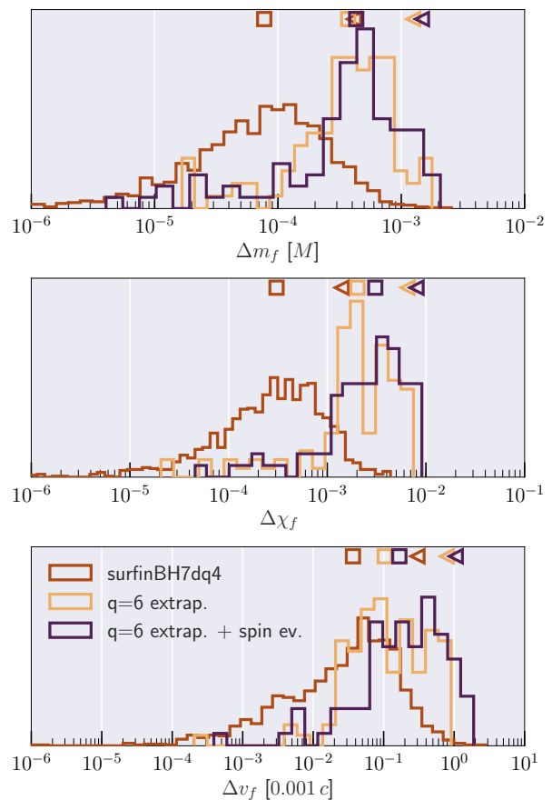
FIG. 11. Error histograms of the remnant mass, spin magnitude and kick magnitude when extrapolating surfinBH7dq4 to mass ratio q = 6 . The training range errors from Fig. 7 are reproduced here for comparison. We show errors using the NR spins at t = -100M (yellow) as well as the initial NR spins (blue) as inputs for the model. The square (triangle) markers indicate median (95th percentile) values.
