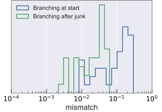
FIG. 14. NR resolution mismatches for the simulation leading to the largest NR mismatch in the left panel of Fig. 4. The different samples in the histogram correspond to comparisons at different angles on the sky. The blue histogram shows the current resolution errors when the two resolutions start with the same initial data at the start of the simulation. All points in the blue histogram are the same as those included in the left panel of Fig. 4. The green histogram shows the resolution errors for the same case when the two resolutions start with the same initial data at \sim 1000M after start, at which point the junk radiation has left the simulation domain.
