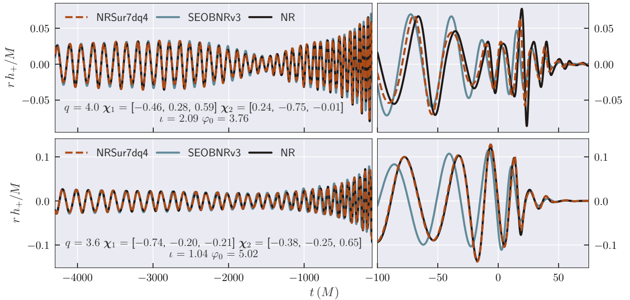
FIG. 5. The plus polarization of the waveforms for the cases that result in the largest mismatch for NRSur7dq4 (top) and SEOBNRv3 (bottom) in the left panel of Fig. 4. We also show the corresponding NR waveforms. Each waveform is projected using all available modes for that model, along the direction that results in the largest mismatch for NRSur7dq4 (SEOBNRv3) in the top (bottom) panel. Note that NRSur7dq4 is evaluated using trial surrogates that are not trained using these cases. The binary parameters and the direction in the source frame are indicated in the figure text. All waveforms are time shifted such that the peak of the total amplitude occurs at t = 0 [using all available modes, according to Eq. (5)]. The waveform modes are then rotated to have their orbital angular momentum aligned with the z -axis, and such that the orbital phase is equal to zero at t = -4300M .
