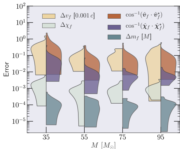
FIG. 8. Errors for surfBH7dq4 in predicting remnant properties when spins are specified at an orbital frequency of f_0 = 10 Hz. For four different total masses, we compute the differences between the surrogate prediction of various remnant properties with the value obtained in the NR simulation. For each mass, these differences are shown as a vertical histogram. Note that the distributions in these plots are normalized to have a fixed height, not fixed area.
