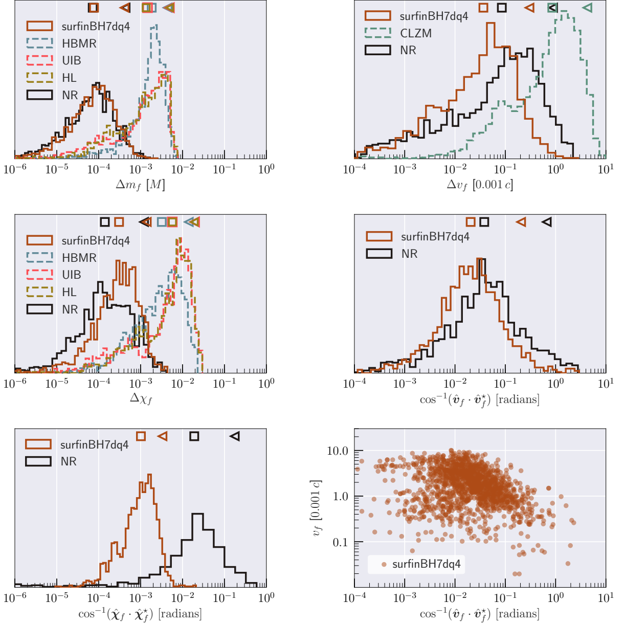
FIG. 7. Error histograms for surfinBH7dq4 for the remnant mass, spin magnitude, spin direction, kick magnitude, and kick direction for precessing BBH with mass ratios q \leq 4 and spin magnitudes \chi_1, \chi_2 \leq 0.8 . The direction error is the angle between the predicted vector and a fiducial vector, taken to be the high-resolution NR case and indicated by *. Square (triangle) markers indicate median (95th percentile) values. Also shown are the NR resolution errors and errors for different existing fitting formulae. In the bottom-right panel we show the joint distribution of kick magnitude and kick-direction error.
