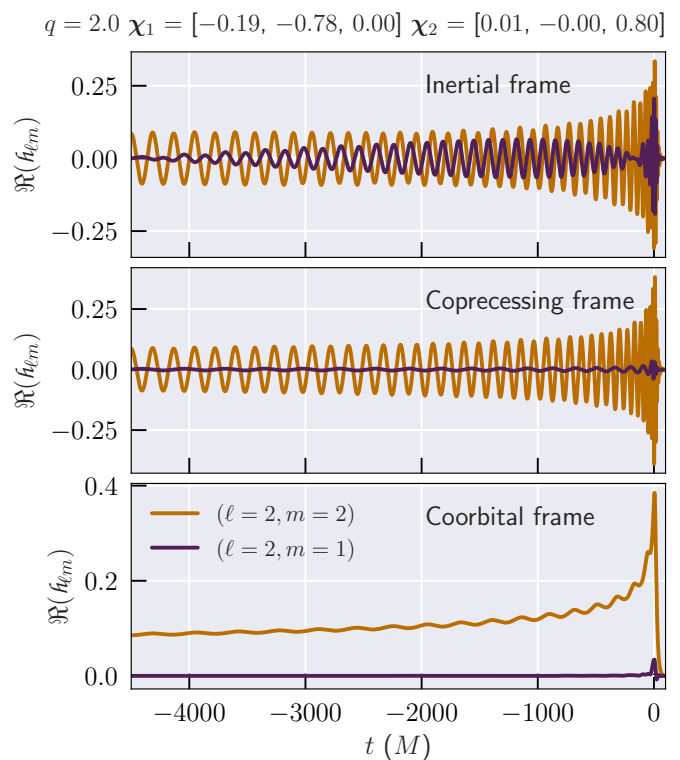
FIG. 1. The real part of the (2, 2) and (2, 1) modes of the gravitational waveform in the inertial (top), coprecessing (middle), and coorbital (bottom) frames. In the inertial frame, the amplitude of the (2, 1) mode can be comparable to that of the (2, 2) mode. In the coprecessing frame, on the other hand, the (2, 2) mode always dominates. In addition, most effects of precession are removed by the rotation and the waveform in the coprecessing frame resembles that of a nonprecessing system. In the coorbital frame, finally, the waveform is further simplified and does not oscillate about zero. Mass ratio and initial spins used to produce this figure are indicated at the top of the plot.
