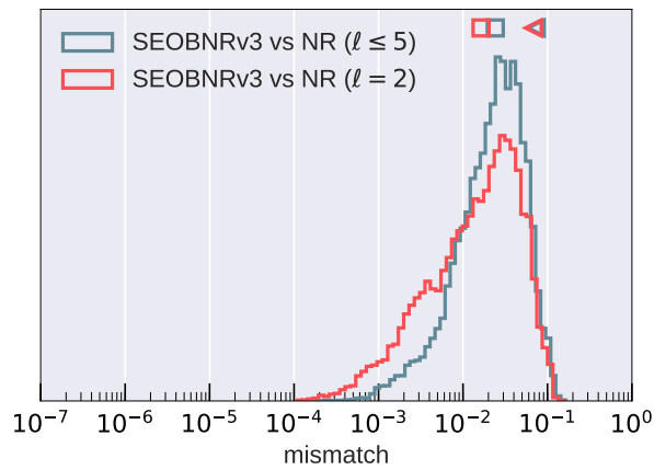
FIG. 6. Same as the left panel of Fig. 4 but using only \ell = 2 modes for NR when compared to SEOBNRv3. The blue histogram from the left panel of Fig. 4, where SEOBNRv3 is compared to NR with all \ell \leq 5 modes, is reproduced here for comparison. The square (triangle) markers at the top indicate the median (95th percentile) values.
