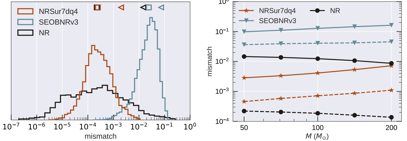
FIG. 4. Mismatches for NRSur7dq4 and SEOBNRv3 models, when compared against precessing NR simulations using all \ell \leq 5 modes with mass ratios q \leq 4 , and spin magnitudes \chi_1, \chi_2 \leq 0.8 . The NRSur7dq4 errors shown are out-of-sample errors. Also shown are the NR resolution errors. Mismatches are computed at several sky locations using all available modes for each model: \ell \leq 4 for NRSur7dq4, and \ell = 2 for SEOBNRv3. The NR error is computed using all \ell \leq 5 modes from the two highest available resolutions. Left panel: Mismatches computed using a flat noise curve. The square (triangle) markers at the top indicate the median (95th percentile) values. Right panel: Mismatches computed using the Advanced LIGO design sensitivity noise curve, as a function of total mass. The dashed (solid) lines indicate the median (95th percentile) values over different NR simulations and points in the sky.
