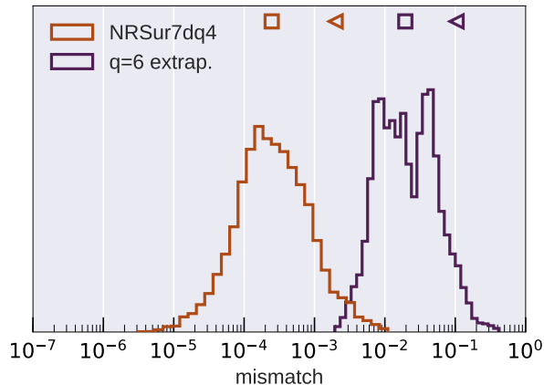
FIG. 10. Mismatch histogram when extrapolating the NR-Sur7dq4 waveform model to mass ratio q = 6 . The mismatches are computed using a flat noise curve. The training range errors from the left panel of Fig. 4 are reproduced here for comparison. The square (triangle) markers indicate median (95th percentile) values.
