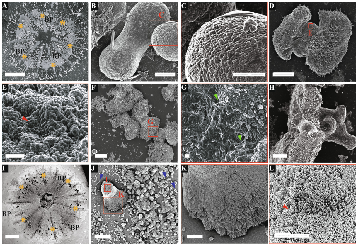
Fig. 1. Early mineral structures in Stylophora pistillata and Pocillopora acuta primary polyps. SEM micrographs of the mineral deposit structures of 3 days settled S. pistillata (A–H) and P. acuta (I–L), using an in-lens secondary electron detector. (A, I) Primary polyps of S. pistillata and P. acuta respectively, after removal of the tissue. (B) S. pistillata pristine dumbbells. (C) Higher magnifications of the region depicted in a red box in B showing that the pristine dumbbell is characterized by nano-granules. (D) S. pistillata mineral deposition in a developing dumbbell like shape (E) Higher magnification of the region depicted in the red box in (D) The surface structure of the center of the dumbbell showing nano-granules (red Arrowhead). (F) Merged dumbbells connected by needle shaped crystals. The structure is part of a secondary septum. (G) High magnification of the region depicted in the red box in (F), shows that the edges of the dumbbell are composed of needle shaped crystals embedded with organic fibers (green arrowheads) (H) A dumbbell, located on the septum wall elevated from the basal plate plane. (I) P. acuta dumbbell basal plate seemingly merging with small rod-shaped structures also forming the septum. (J) P. acuta rods (blue arrowheads) and dumbbell-like mineral deposit (K) Needle shaped crystals at the opposite end of the dumbbell. (L) The surface structure of the other end of the dumbbell, made of nano-granular particles (red arrowhead). Orange stars – septa, BP – basal plate. Scale bars: 300 \mu\text{m} (A, I), 2 \mu\text{m} (B, C, K, L), 10 \mu\text{m} (D, F, H, J), 500 nm (E, G). (For interpretation of the references to color in this figure legend, the reader is referred to the web version of this article.)
