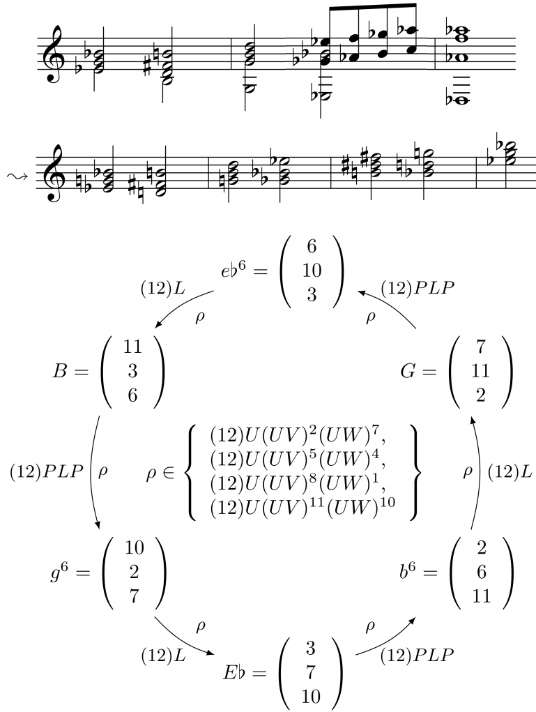
FIGURE 5. The two musical staves show the extrapolation of a hexatonic cycle of alternating root position major triads and first inversion minor triads from the first four chords in the harmonization of Grail motive in Wagner’s Parsifal , Act 3, measures 1098–1100. The top staff depicts David Clampitt’s [4] reduction of these measures. The staff below depicts our hexatonic extrapolation. The hexagonal network provides a transformational analysis of this extrapolation. The outer labels (12)PLP and (12)L denote two contextual transformations between the chosen voicings (i.e. root position major triads and first inversion minor triads). The inner label \rho stands for any of the four elements of \Sigma_3 \times \mathcal{J} that provide a cyclic orbit along these six voicings. The normal forms of these group elements are depicted in the center of the network.
