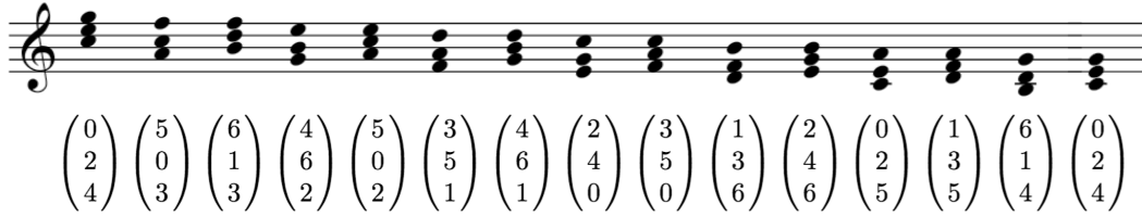
FIGURE 7. The diatonic falling fifth sequence and its encoding as vectors with entries in \mathbb{Z}_7 . The encoding of the C -major scale collection is C \leftrightarrow 0 , D \leftrightarrow 1 , E \leftrightarrow 2 , ..., and finally B \leftrightarrow 6 . The diatonic falling fifth sequence is a cycle of the sole transformation (12)U(UV)^3 in \Sigma_3 \ltimes \mathcal{J}(\mathbb{Z}_7) .
