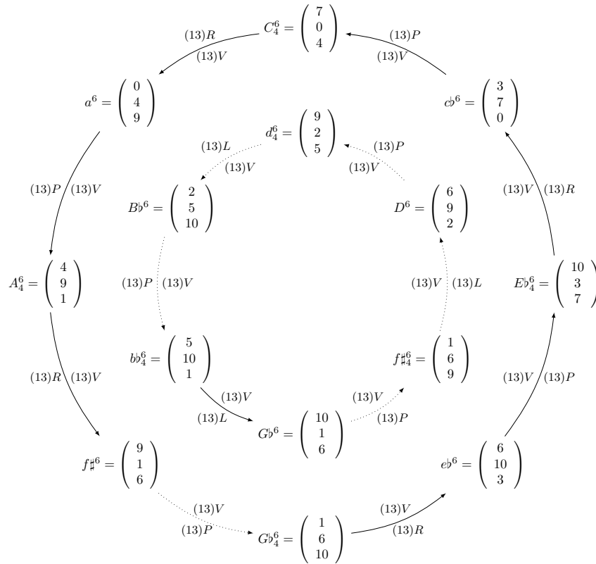
(B) Cyclic networks extrapolating connections between triadic segments in Schoenberg, String Quartet in D minor, op. 7, measures 88–93. The outer cycle is the octatonic PR -cycle of the first 9 triadic segments of Figure 6a, while the inner cycle is the hexatonic PL -cycle implied by the final viola L -relationship bb_4^6 \mapsto Gb^6 and the P -relationship between the final Gb and the earlier f\sharp in the 2nd violin. All implied edges are indicated by dotted arrows.
