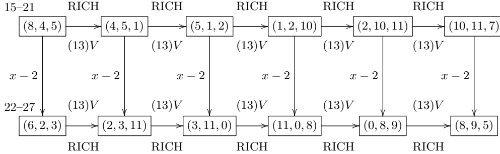
FIGURE 3. Interpretation of Webern, Concerto for Nine Instruments, op. 24, Second Movement, measures 15–21 and 22–27. Each 3-note sequence is a permutation of some transposition/inversion of \{0, 1, 4\} . The rows are connected by retrograde inversion enchainning, abbreviated RICH. The pattern terminates after 6 sequences, but could continue to 8 sequences to traverse a complete cycle that exhausts the octatonic \{1, 2, 4, 5, 7, 8, 10, 11\} by Corollary 6.2 of [17].
