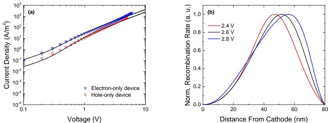
Fig. 2 | Charge transport in CzDBA and simulated recombination profile. (a) Current density-voltage characteristics of CzDBA electron- and hole-only devices (symbols) with a CzDBA layer thickness of 155 nm. Solid lines are fits with a numerical drift-diffusion model. (b) Normalized recombination profile simulated for an 80 nm CzDBA OLED at different driving voltages.
