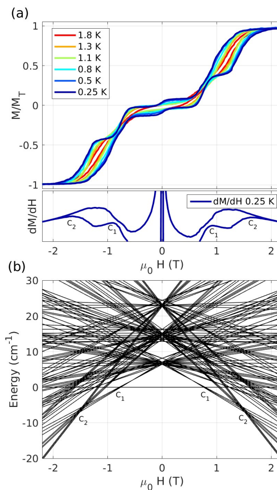
Fig. 3 (a) Applied field dependence of single-crystal Hall bar magnetisation, measured for various temperatures within the molecular X-Y plane with a magnetic field sweep rate of 20 mT/sec. At 0.25 K two clear steps in the magnetisation are observed, most clearly are identified as maxima in dM/dH (labelled c_1 and c_2 ), on increasing magnitude of applied field. (b) Zeeman diagram corresponding with data in (a) based on Hamiltonian (1).
