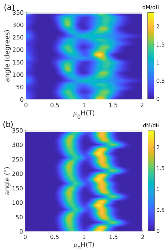
Fig. 4 Measured (a) and calculated (b) first derivative of magnetisation (dM/dH) plotted as a function of sample orientation within the molecular X-Y plane at 0.3 K. An angle of zero corresponds with the magnetic field vector at 45° from the molecular X and Y axes. Maxima in dM/dH for a given angle correspond with field crossings referred to in the text as c_1 and c_2 . Calculations are based on Hamiltonian (1) described within the text.
