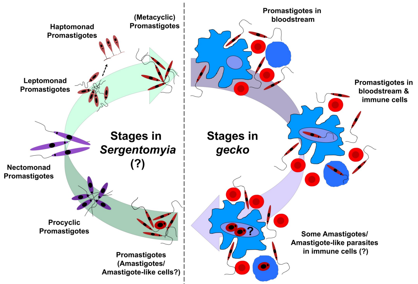
Fig 2. Simplified life cycle of L. tarentolae ( Sauroleishmania ). Sand fly ( Sergentomyia ) takes a blood meal from a gecko and thereby ingests promastigotes (major form) and some amastigotes/amastigote-like cells (minor form) of L. tarentolae . Inside the gut of the sand fly, immune cells burst, and the phagocytized part of Leishmania is released. Promastigotes colonize the lumen of the cloaca, the intestine (hindgut), and rarely, the blood of the sand fly. Although not known, it is possible that promastigotes (and amastigotes) of L. tarentolae undergo several transformations inside the sand fly, with stages of procyclic, nectomonad, leptomonad, haptomonad, and subsequently, metacyclic promastigotes (stages adapted from [80]). Metacyclic promastigotes would be the gecko-infective stage, and they are transferred back to a gecko during a new blood meal. Inside the gecko, promastigotes mainly live free in the blood. A small part is probably phagocytized by immune cells (monocytes and macrophages). Phagocytosed promastigotes might change back into amastigotes/amastigote-like cells, and the life cycle repeats. Immune cells are represented in blue, and erythrocytes are represented in red.
